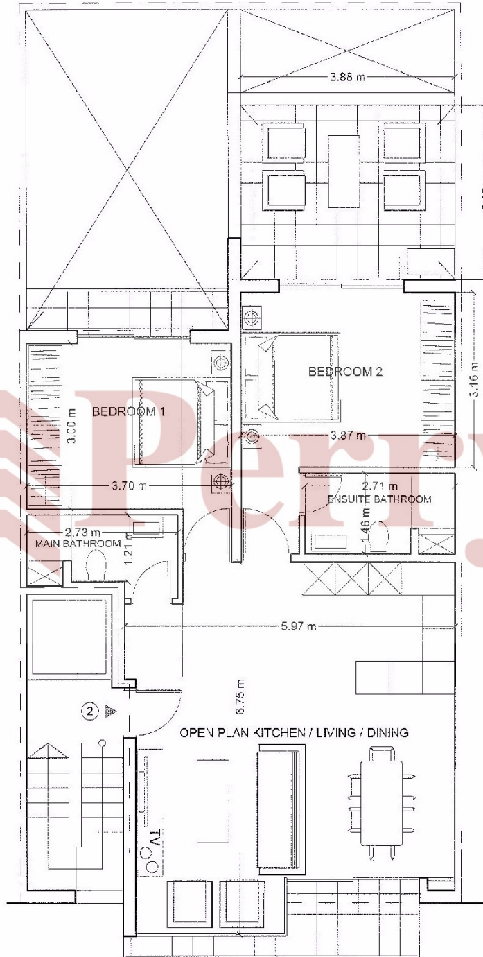
FIRST FLOOR LEVEL PLAN LEVEL 2
