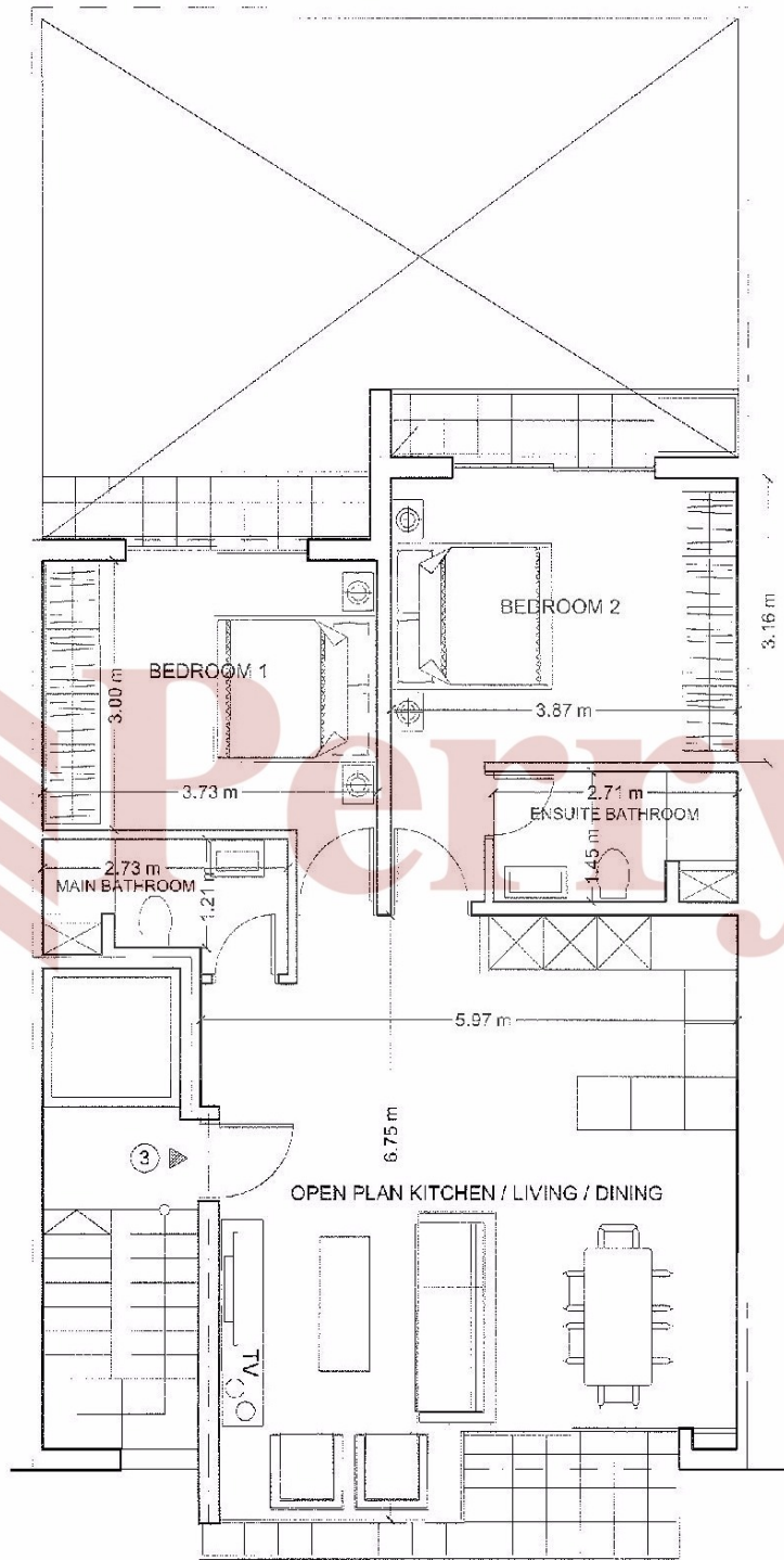
SECOND FLOOR LEVEL PLAN LEVEL 3
