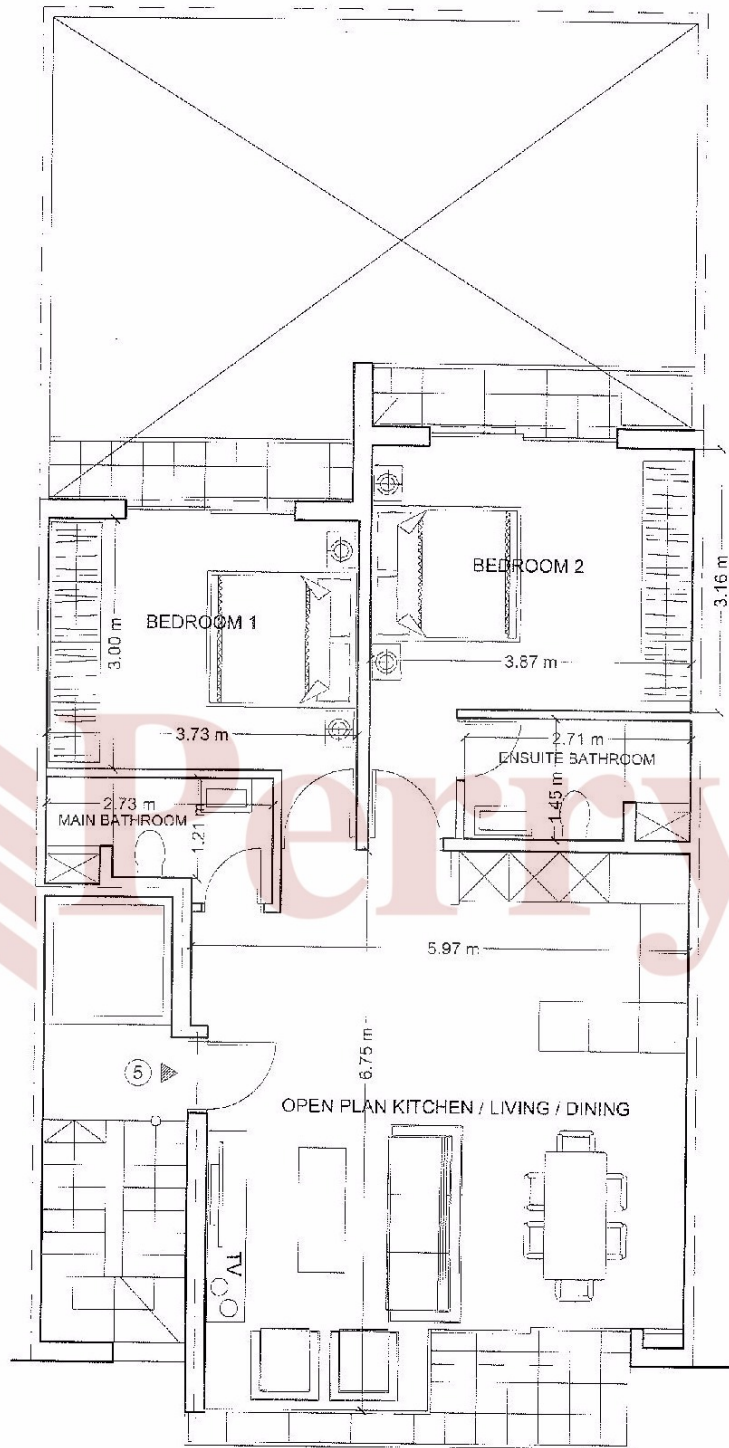
FOURTH FLOOR LEVEL PLAN LEVEL 5
