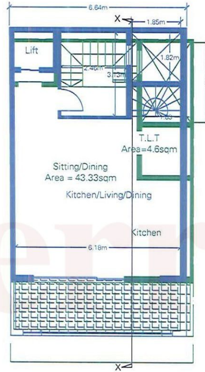
Approved/Existing Receded Floor Plan as per Scale 1:100
