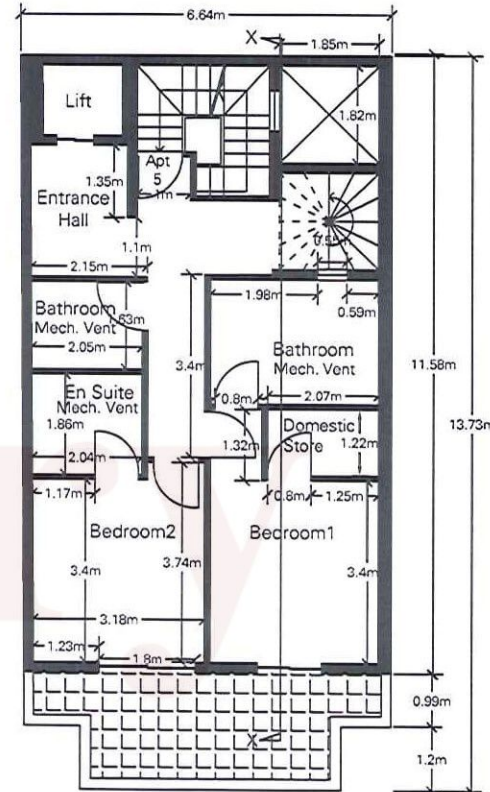
Existing Fifth Floor Plan Scale 1:100
