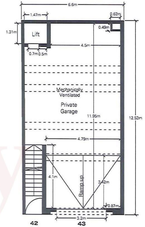
Existing Semi-Basement Floor Plan Scale 1:100
