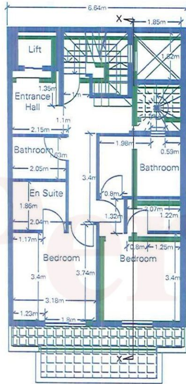
Existing Fifth Floor Plan Scale 1:100
