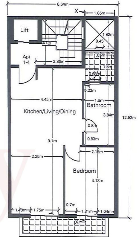
Existing First, Second, Third and Fourth Floor Plans Scale 1:100
