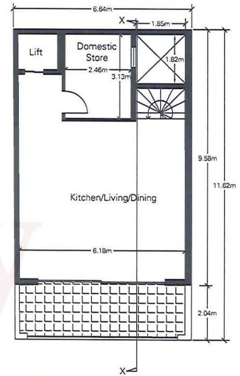
Existing Receded Floor Plan Scale 1:100
