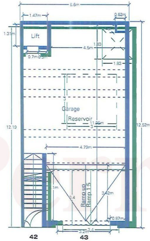
Existing Semi-Basement Floor Plan Scale 1:100
