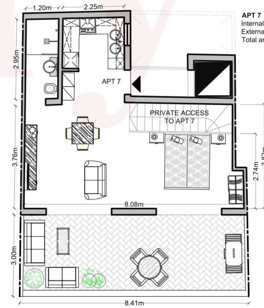
Fifth Floor 1:100
