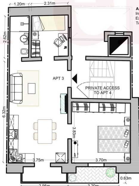
Fourth Floor 1:100
