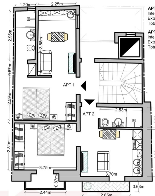
Second Floor 1:100
