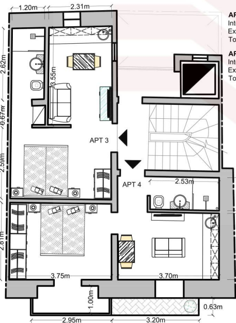
Third Floor 1:100
