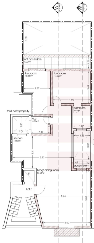
PROPOSED THIRD FLOOR PLAN Scale 1:100
