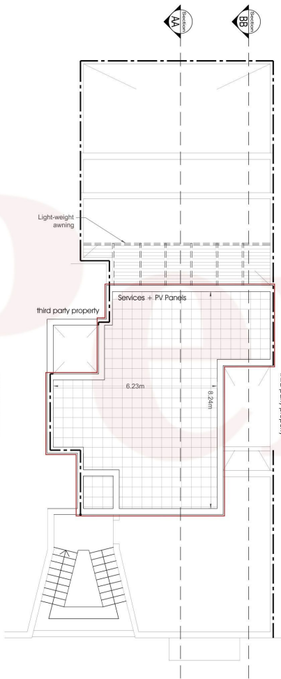
PROPOSED TOP ROOF FLOOR PLAN Scale 1:100
