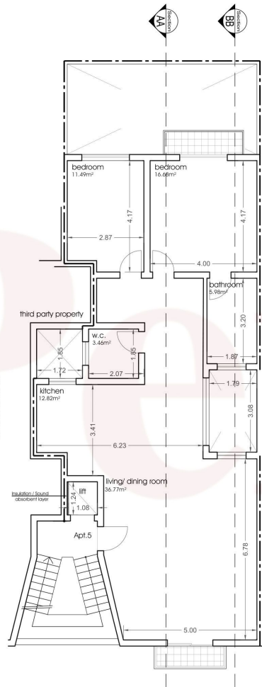
APPROVED/ PROPOSED SECOND FLOOR PLAN Scale 1:100
