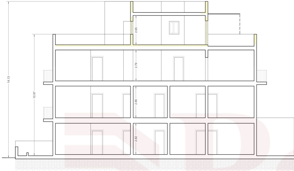
APPROVED SECTION AA Scale 1:100
