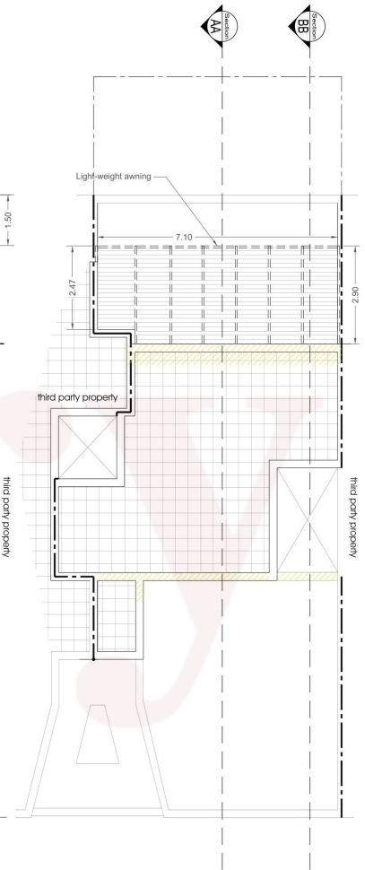
APPROVED ROOF PLAN Scale 1:100
