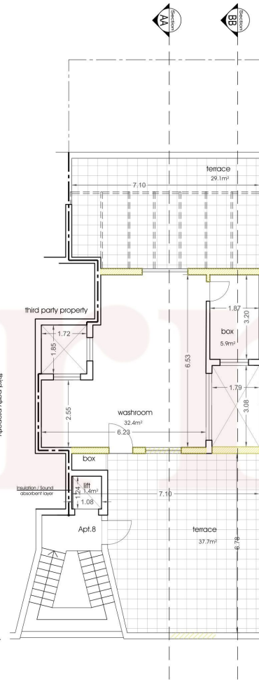
APPROVED SETBACK FLOOR PLAN Scale 1:100
