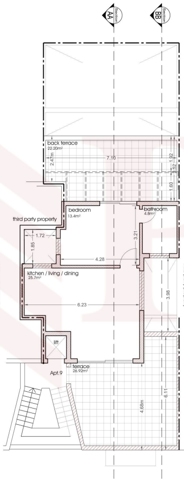
PROPOSED SETBACK FLOOR PLAN Scale 1:100
