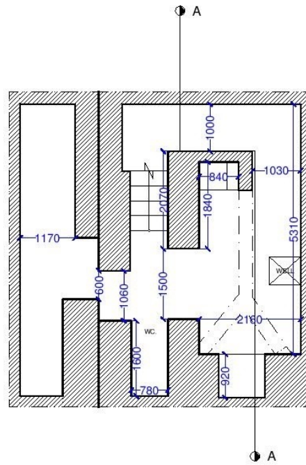
EXISTING BASEMENT PLAN 1:100
