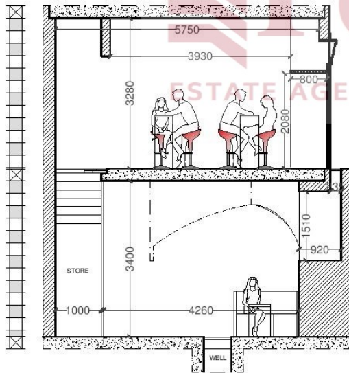
PROPOSED SECTION A - A 1:100
