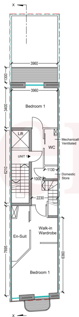
PROPOSED 1ST FLR PLAN Scale 1:100
