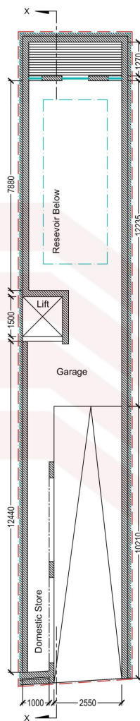
PROPOSED BASEMENT PLAN Scale 1:100
