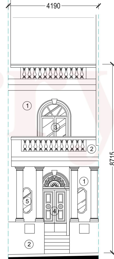
EXISTING ELEVATION
