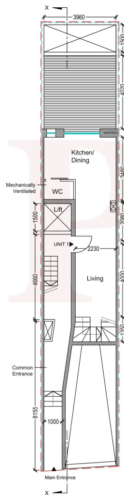
PROPOSED GRND FLR PLAN Scale 1:100
