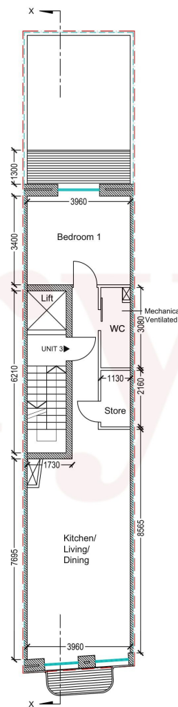
PROPOSED 3RD FLR PLAN Scale 1:100
