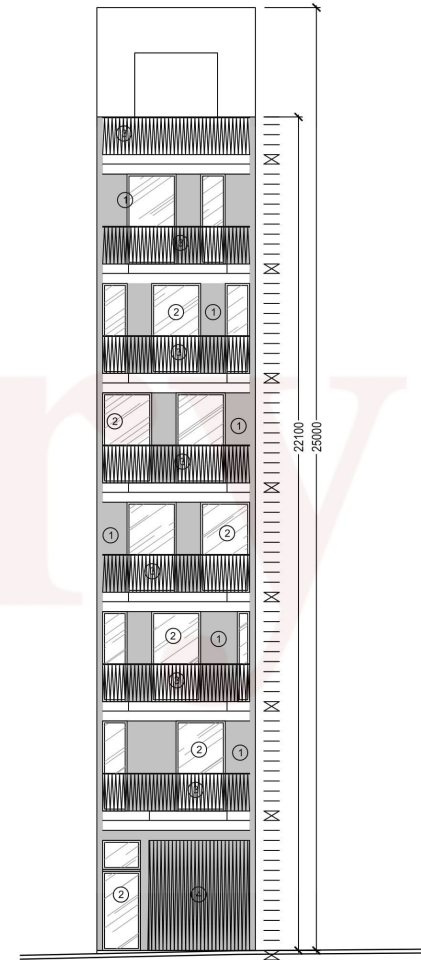
PROPOSED ELEVATION Scale 1:100
