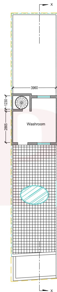
EXISTING ROOF PLAN Scale 1:100
