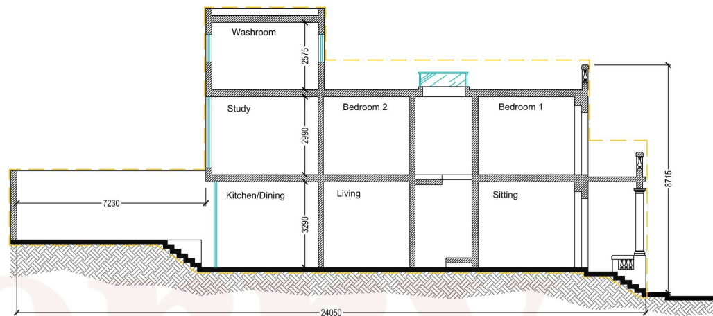
EXISTING SECTION XX Scale 1:100
