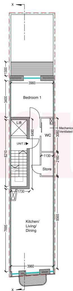
PROPOSED 2ND FLR PLAN Scale 1:100
