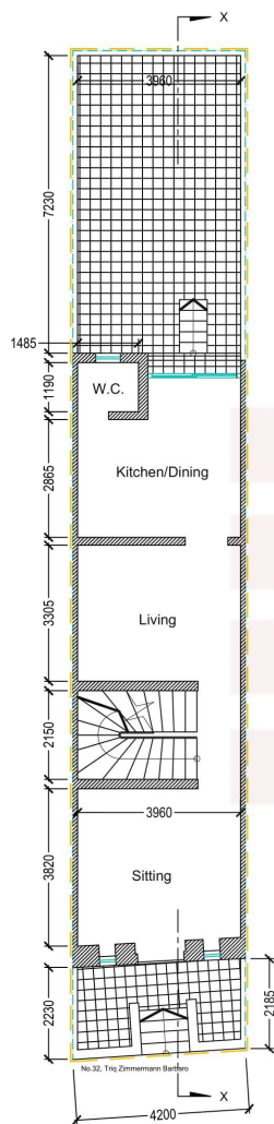
EXISTING GROUND FLR PLAN Scale 1:100
