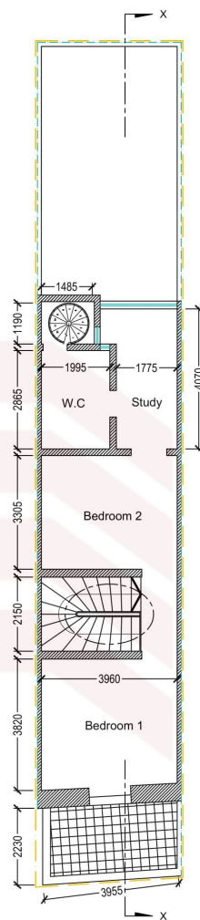
EXISTING FIRST FLR PLAN Scale 1:100
