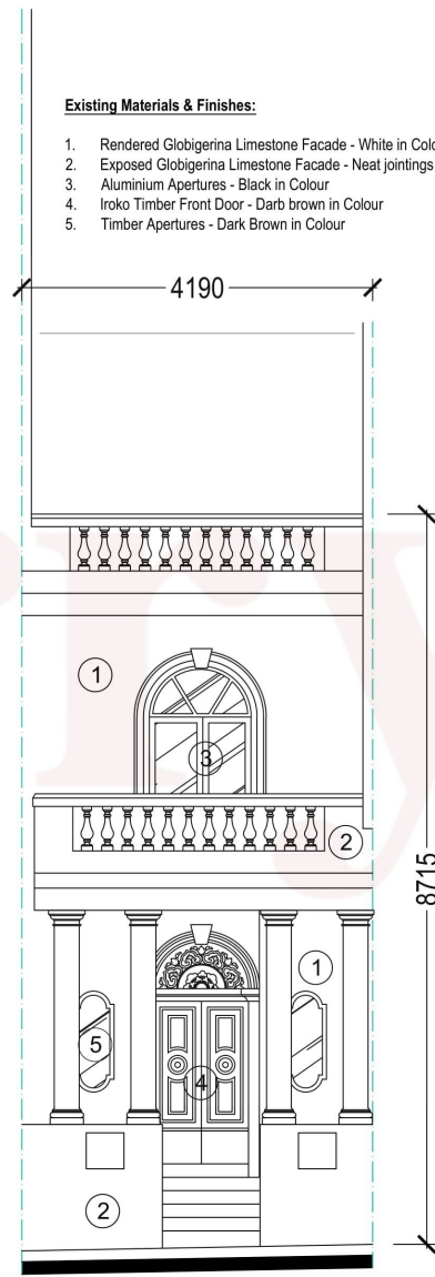
EXISTING ELEVATION Scale 1:50
