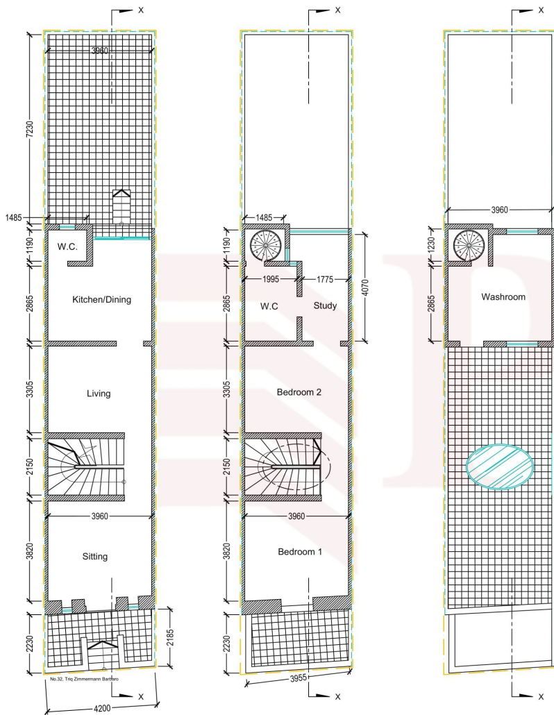
EXISTING GROUND FLR PLAN Scale 1:100
