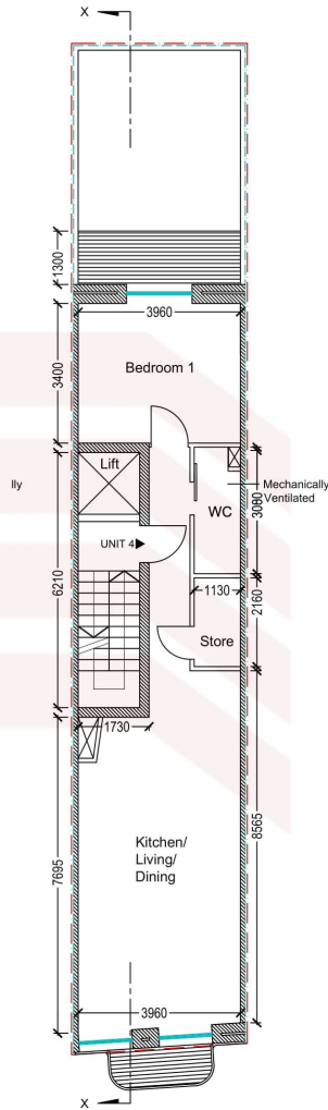
PROPOSED 4TH FLR PLAN Scale 1:100
