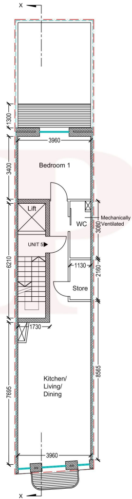
PROPOSED 5TH FLR PLAN Scale 1:100
