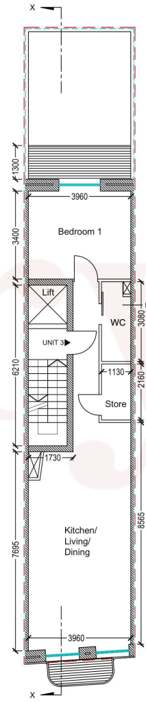
PROPOSED 3RD FLR PLAN Scale 1:100
