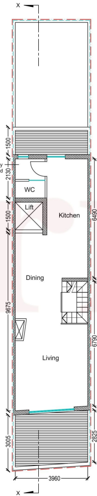
PROPOSED 7TH FLR PLAN Scale 1:100
