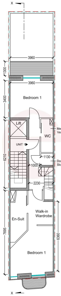
PROPOSED 1ST FLR PLAN Scale 1:100
