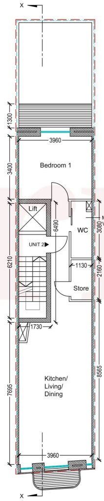
PROPOSED 2ND FLR PLAN Scale 1:100
