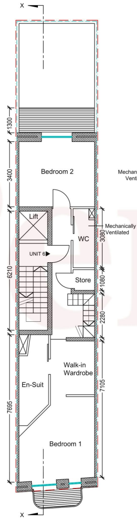
PROPOSED 6TH FLR PLAN Scale 1:100
