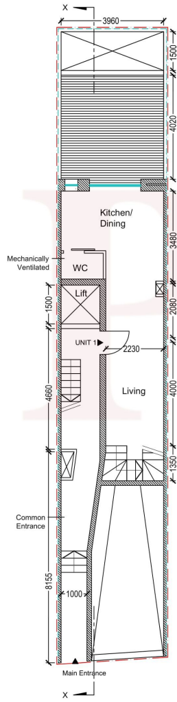
PROPOSED GRND FLR PLAN Scale 1:100
