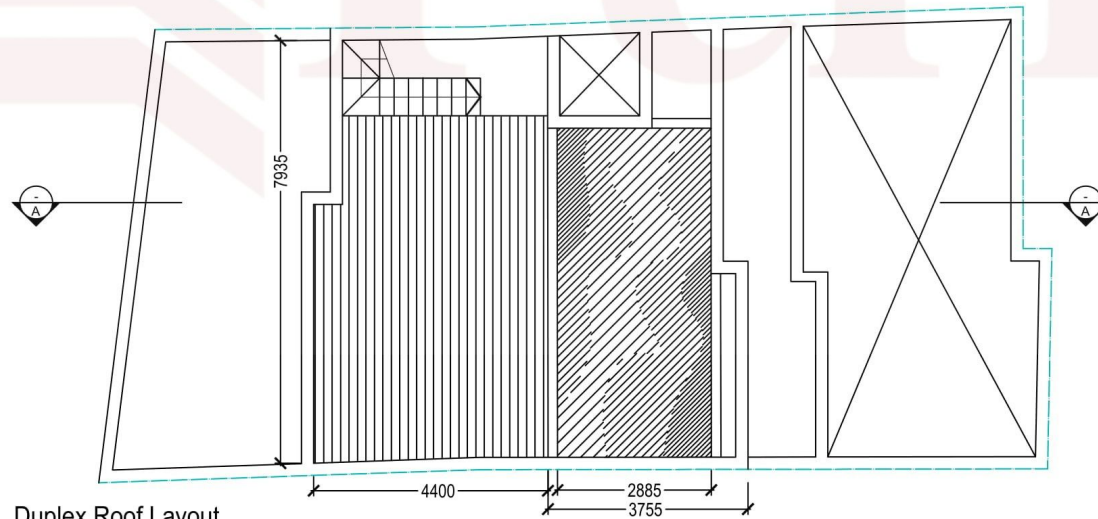
Duplex Roof Layout Scale 1:100
