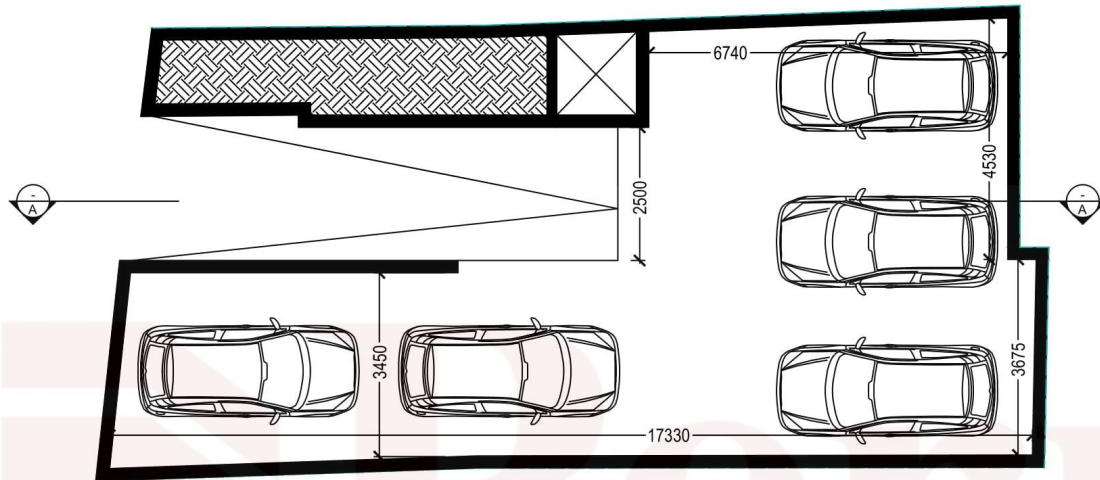
Garage Layout Scale 1:100
