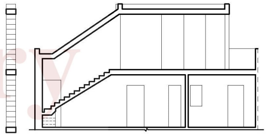
Section through Y-Y
