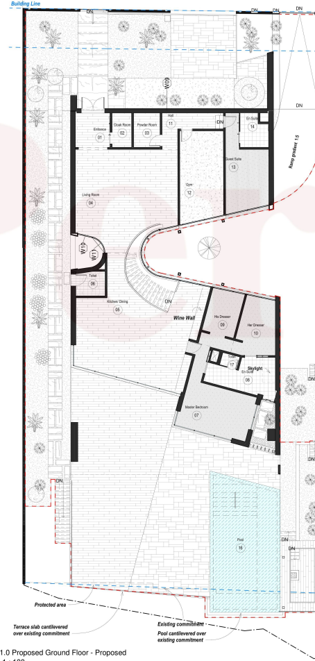
2 1.0 Proposed Ground Floor - Proposed 1 : 100
