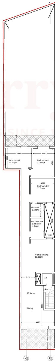
Proposed Receded Floor (Apt 6) Scale 1:100 GFA = 127sqm internal 25.1sqm external
