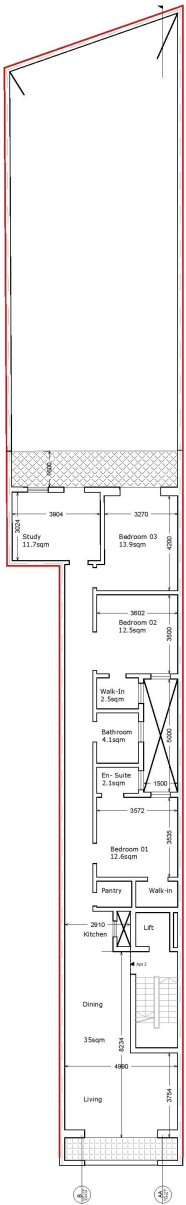
Proposed Second Floor Plan (Apt 2) Scale 1:100 GFA = 134.4m internal 16.2sqm external
