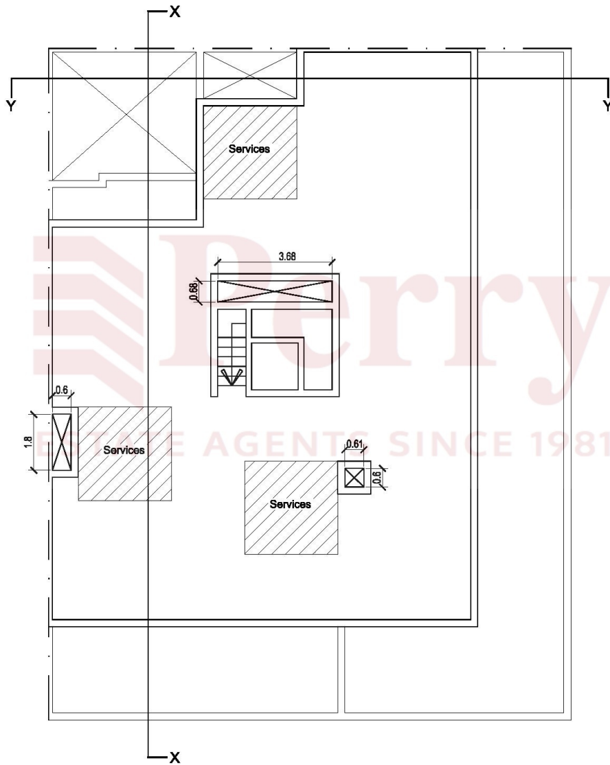
ROOF PLAN
