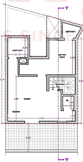
PROPOSED 6th FLOOR PLAN (54.6m 2 & 20.84m 2 ext) Scale:- 1:100
