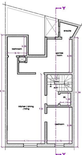
PROPOSED 2nd FLOOR PLAN (78.6m 2 ) Scale:- 1:100
