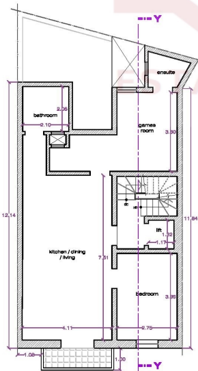
PROPOSED 4th FLOOR PLAN (78.6m 2 Int & 4.15m 2 ext) Scale:- 1:100
