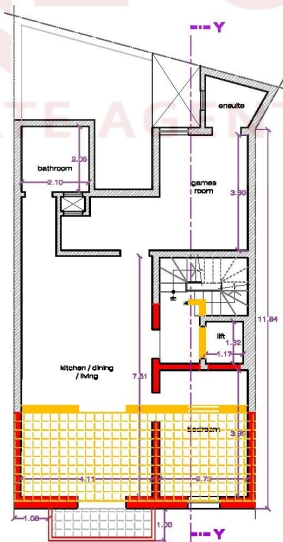
PROPOSED 5th FLOOR PLAN (78.6m 2 Int & 4.15m 2 ext) Scale:- 1:100
