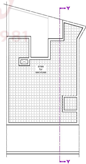
PROPOSED ROOF FLOOR PLAN Scale:- 1:100
