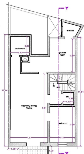
PROPOSED 3rd FLOOR PLAN (78.6m 2 & 4.15m 2 ext) Scale:- 1:100
