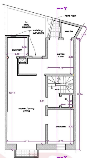
PROPOSED 1st FLOOR PLAN (77.3m 2 & 4.15m 2 ext) Scale:- 1:100
