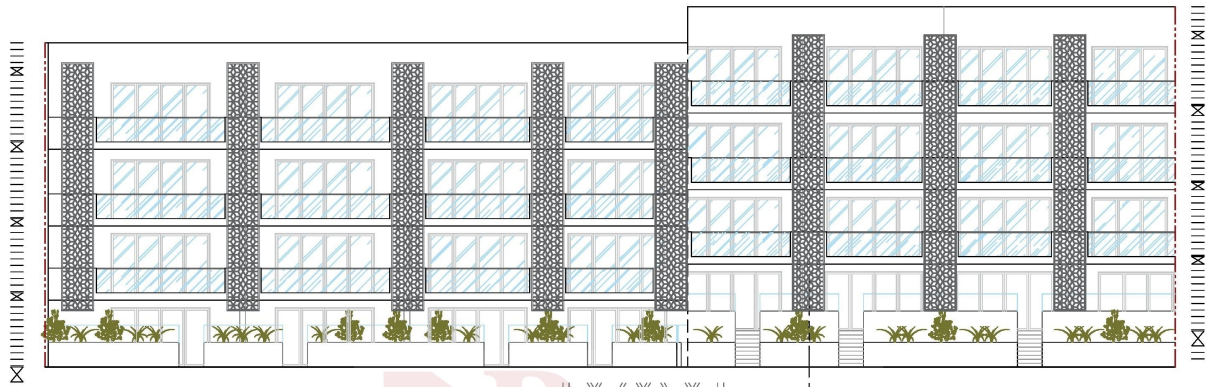
PROPOSED BACK ELEVATION overlooking pool 1:100
