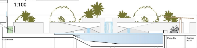
Proposed Section CC 1:100
