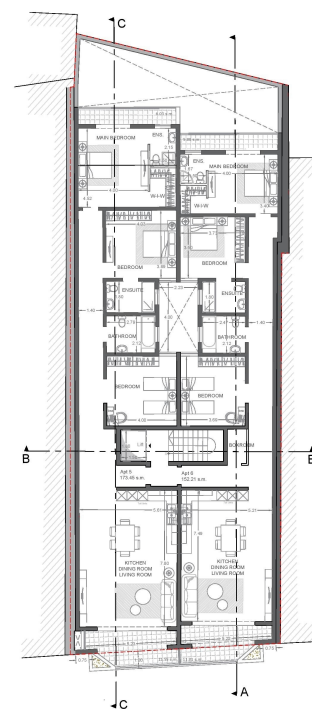
Proposed Second Floor Level
