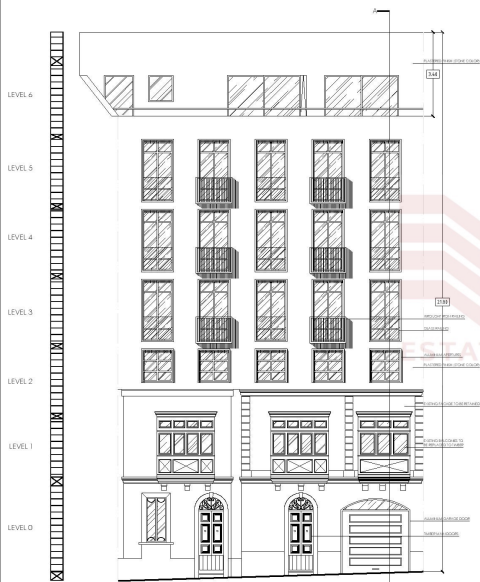
PROPOSED ELEVATION SCALE 1:100
