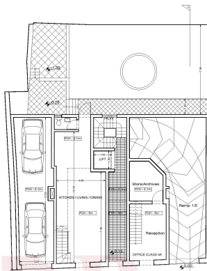
PROPOSED LEVEL 0 Scale: 1/100
