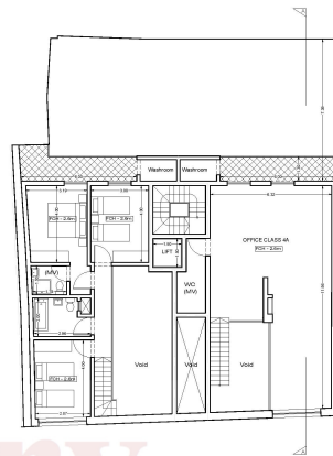
PROPOSED Intermediate LEVEL Scale: 1/100
