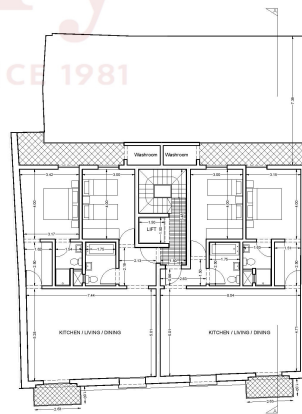
PROPOSED LEVEL 3 Scale: 1/100
