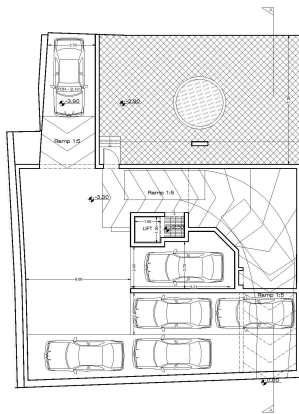
PROPOSED LEVEL -1 Scale: 1/100
