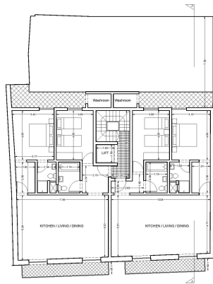
PROPOSED LEVEL 4 Scale: 1:100
