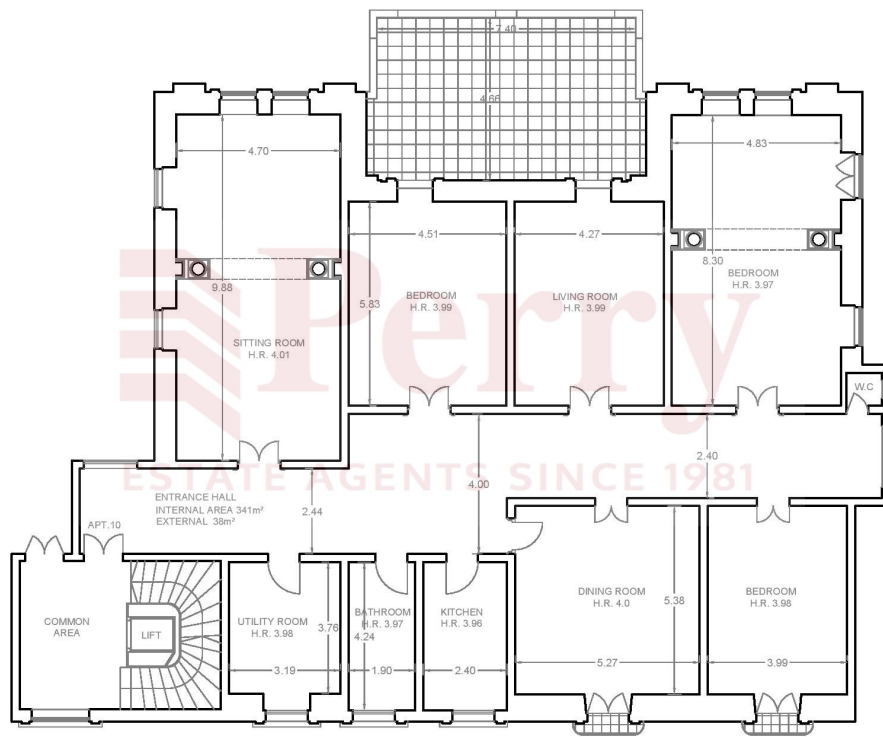
EXISTING SECOND FLOOR PLAN SCALE 1:100
