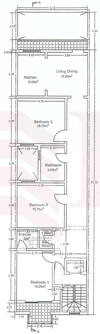
Existing / Proposed First Floor Plan Scale 1:100
