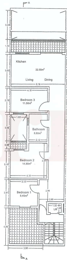
Proposed Receded Floor Plan Scale 1:100
