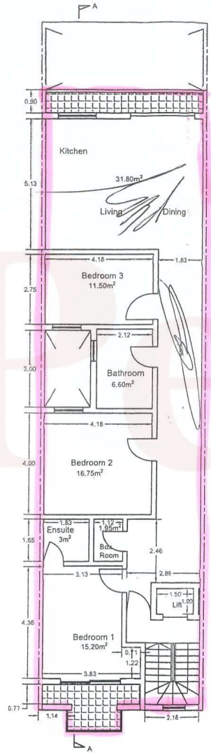
Proposed Second and Third Floor Plan Scale 1:100
