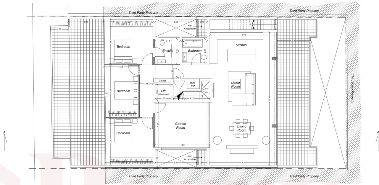
As Approved Level 6 Scale 1:100
