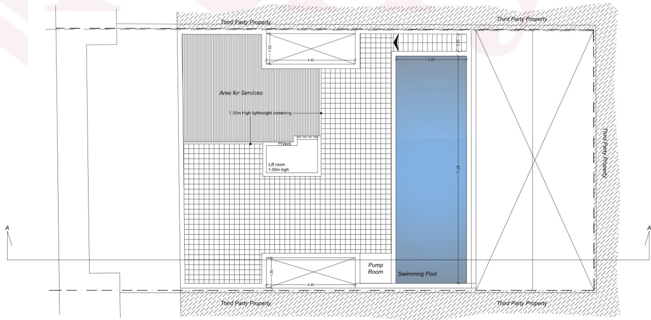
As Proposed Level 7 Scale 1:100
