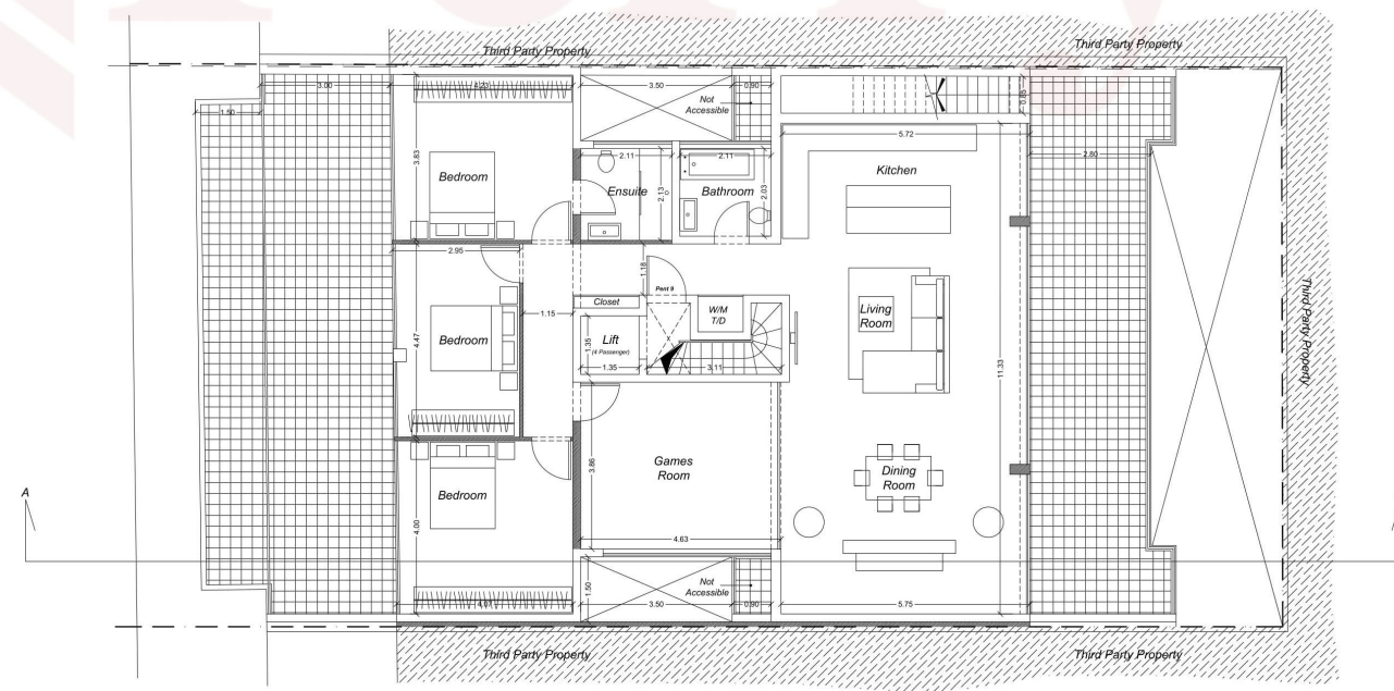
As Proposed Level 6 Scale 1:100
