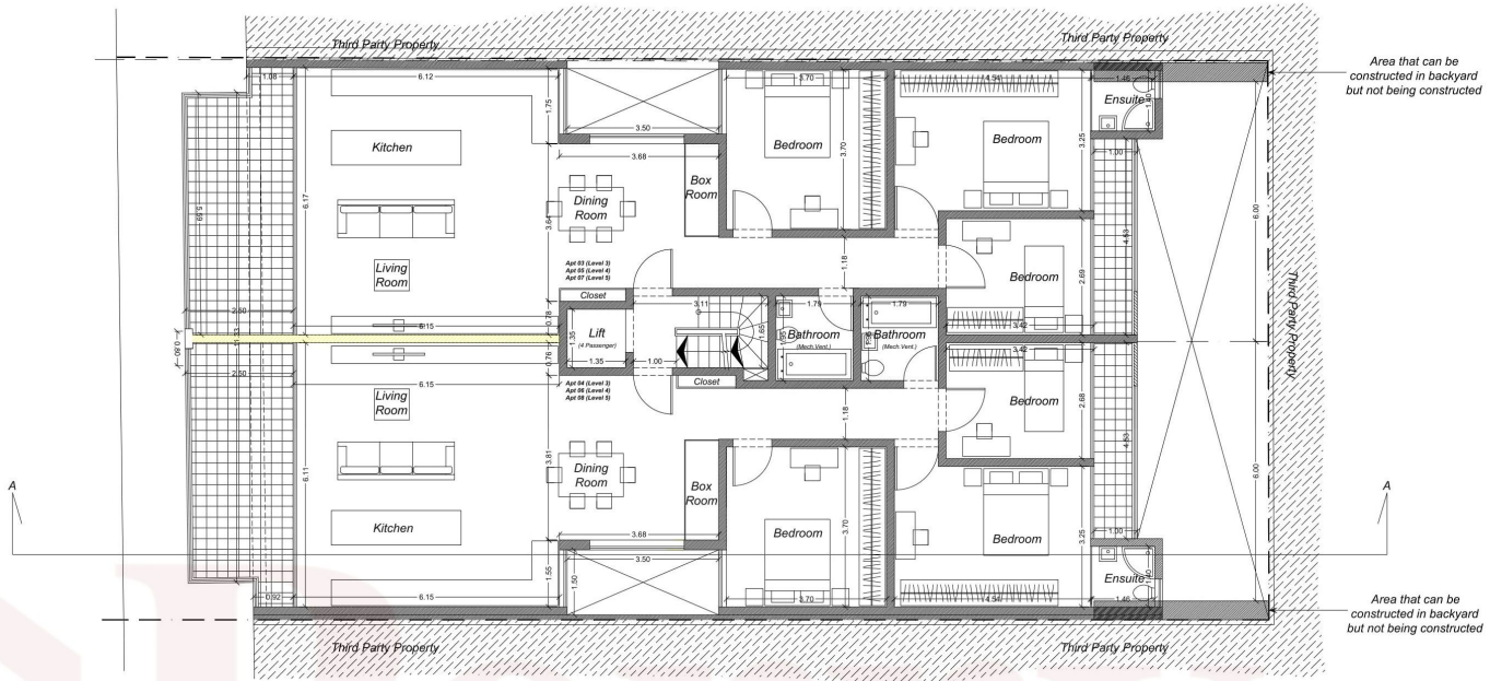
As Approved Levels 3, 4, 5 Scale 1:100
