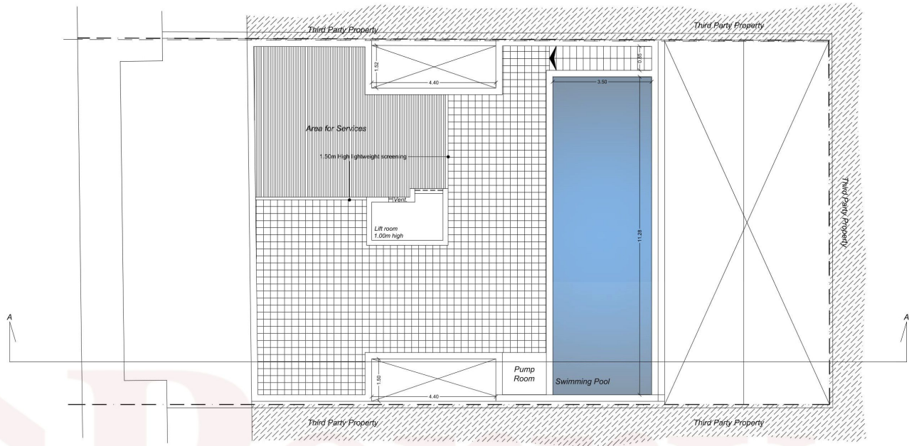
As Approved Level 7 Scale 1:100
