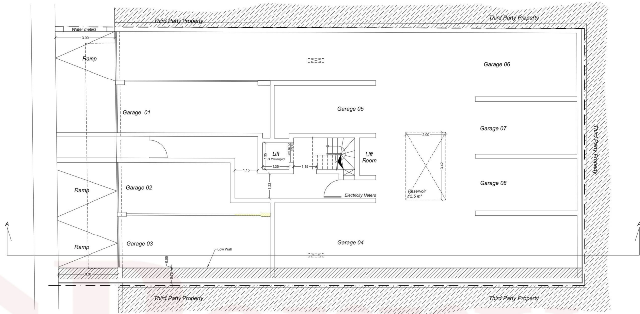
As Approved Level 1 Scale 1:100
