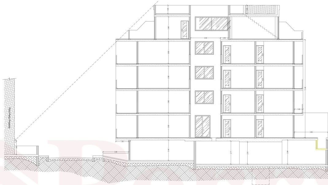
As Approved Section A-A Scale 1:100
