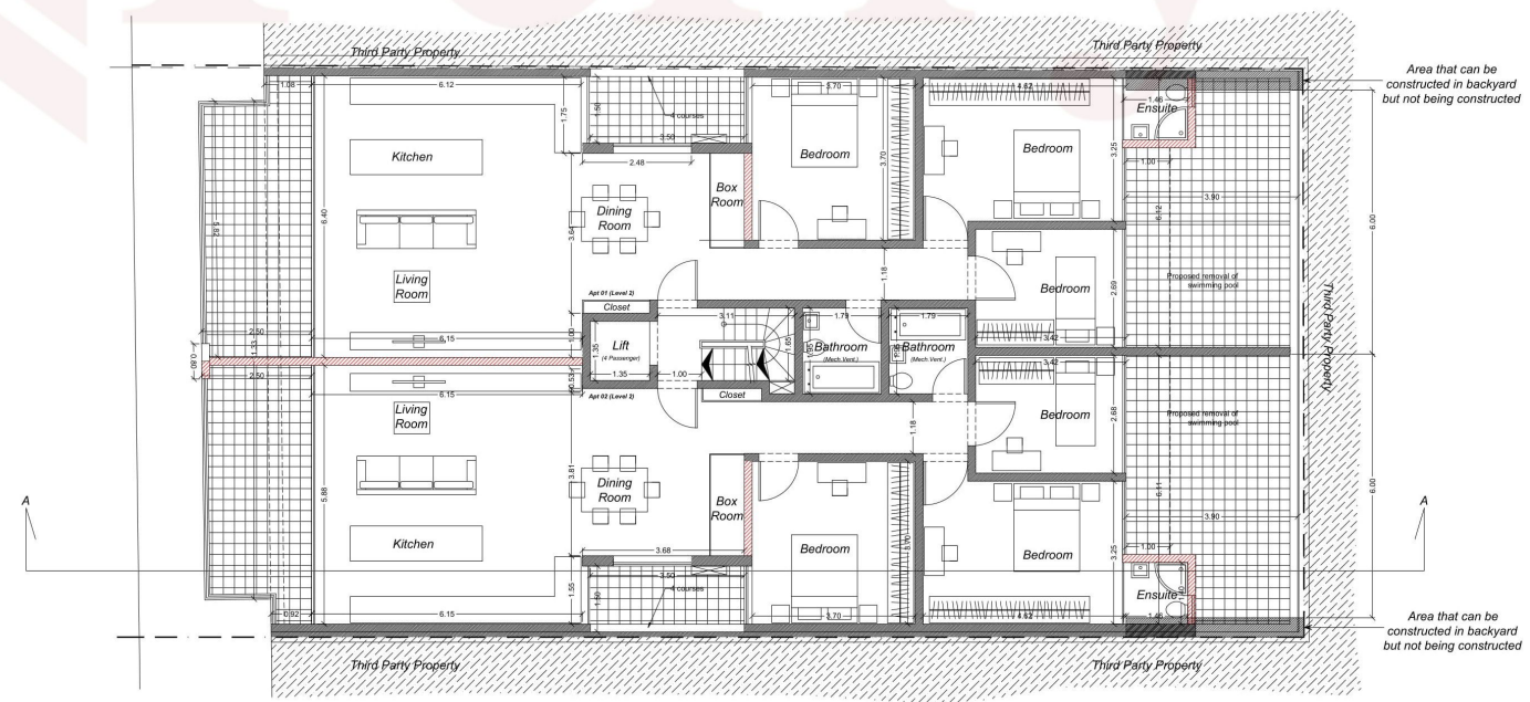
As Proposed Level 2 Scale 1:100
