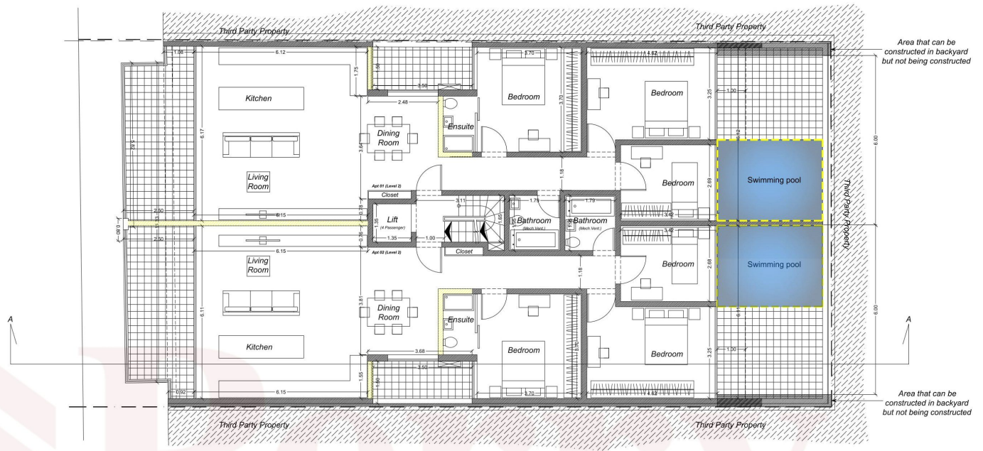
As Approved Level 2 Scale 1:100
