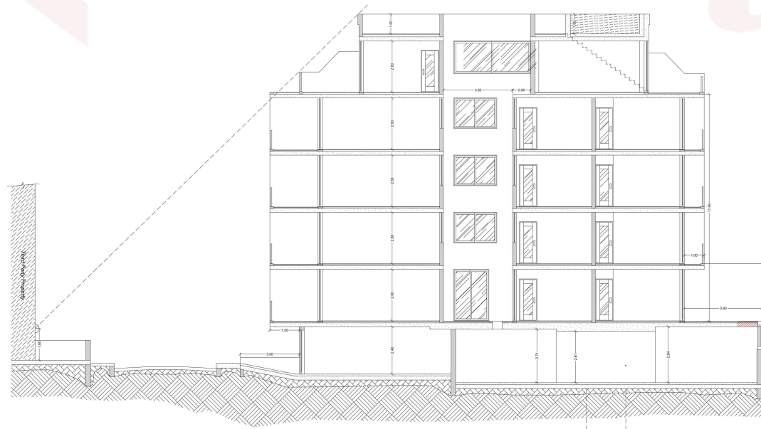
As Proposed Section A-A Scale 1:100
