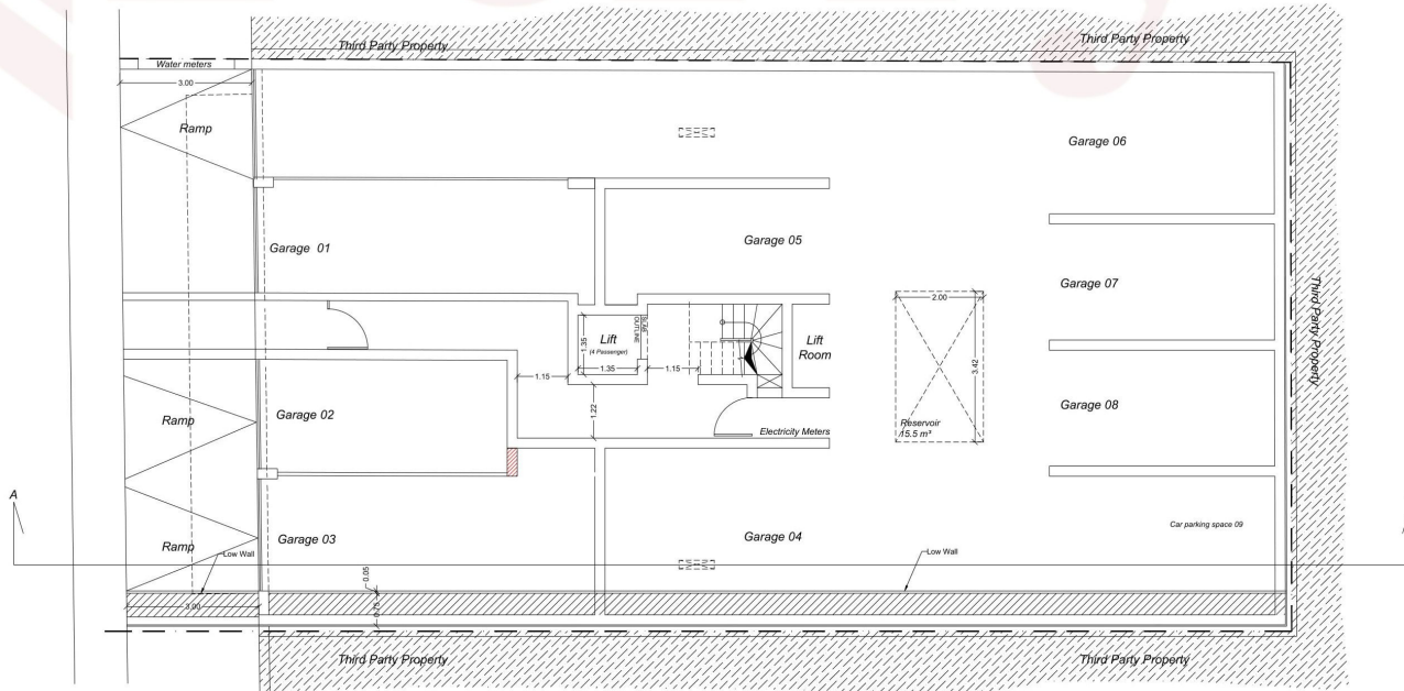
As Proposed Level 1 Scale 1:100
