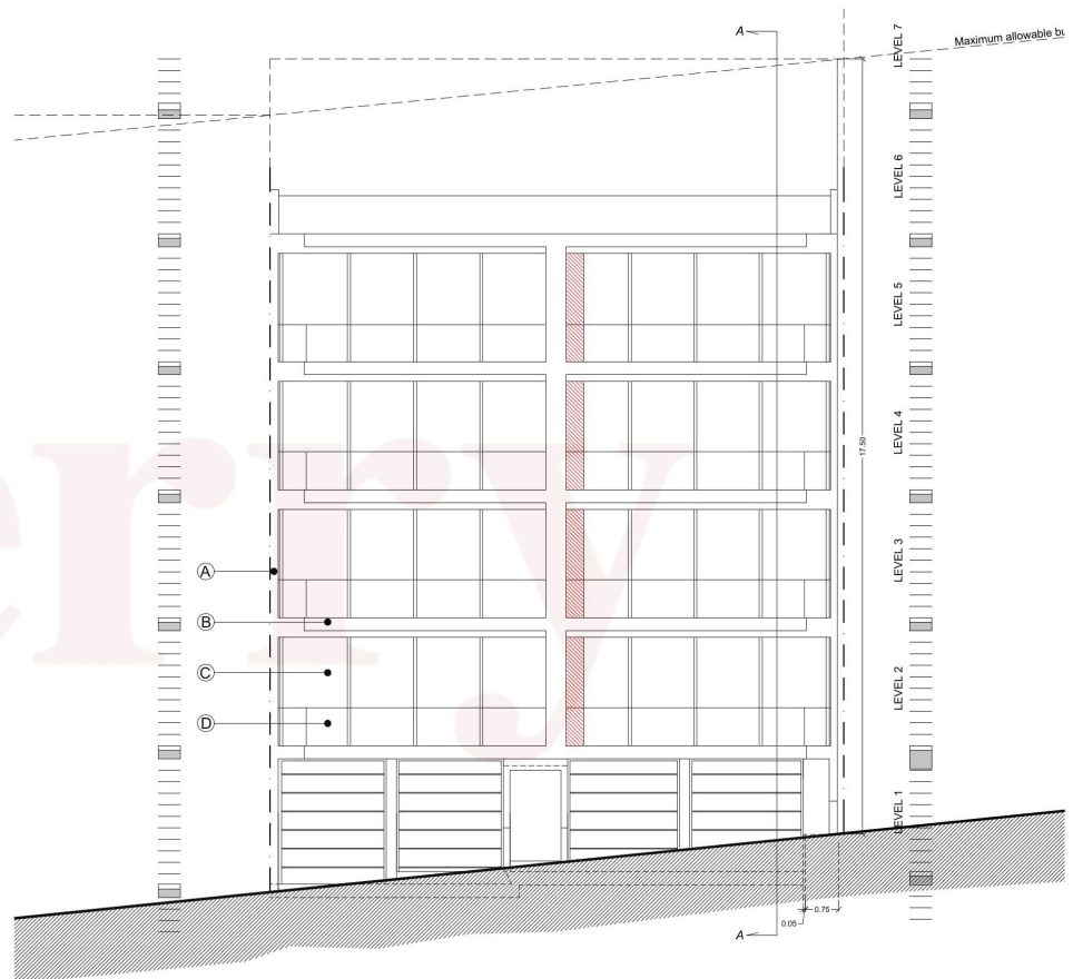
As Proposed Elevation Scale 1:100
