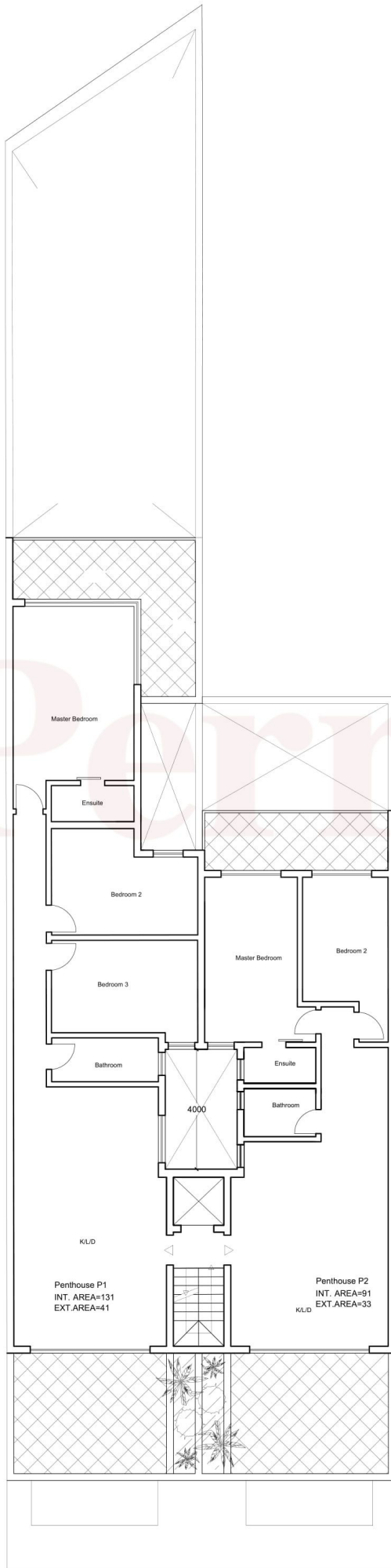
PROPOSED PENTHOUSE
