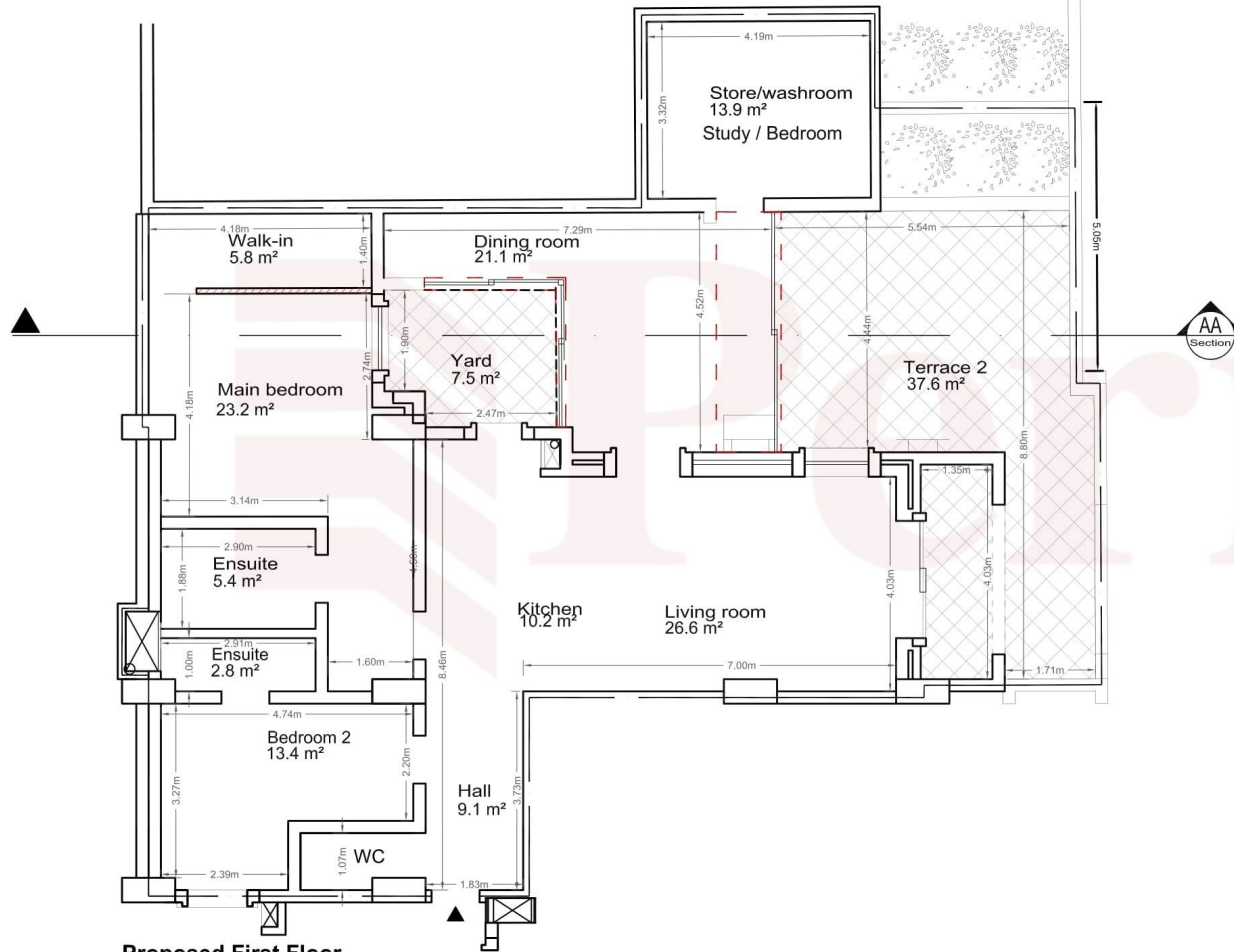
Proposed First Floor Scale 1:100
