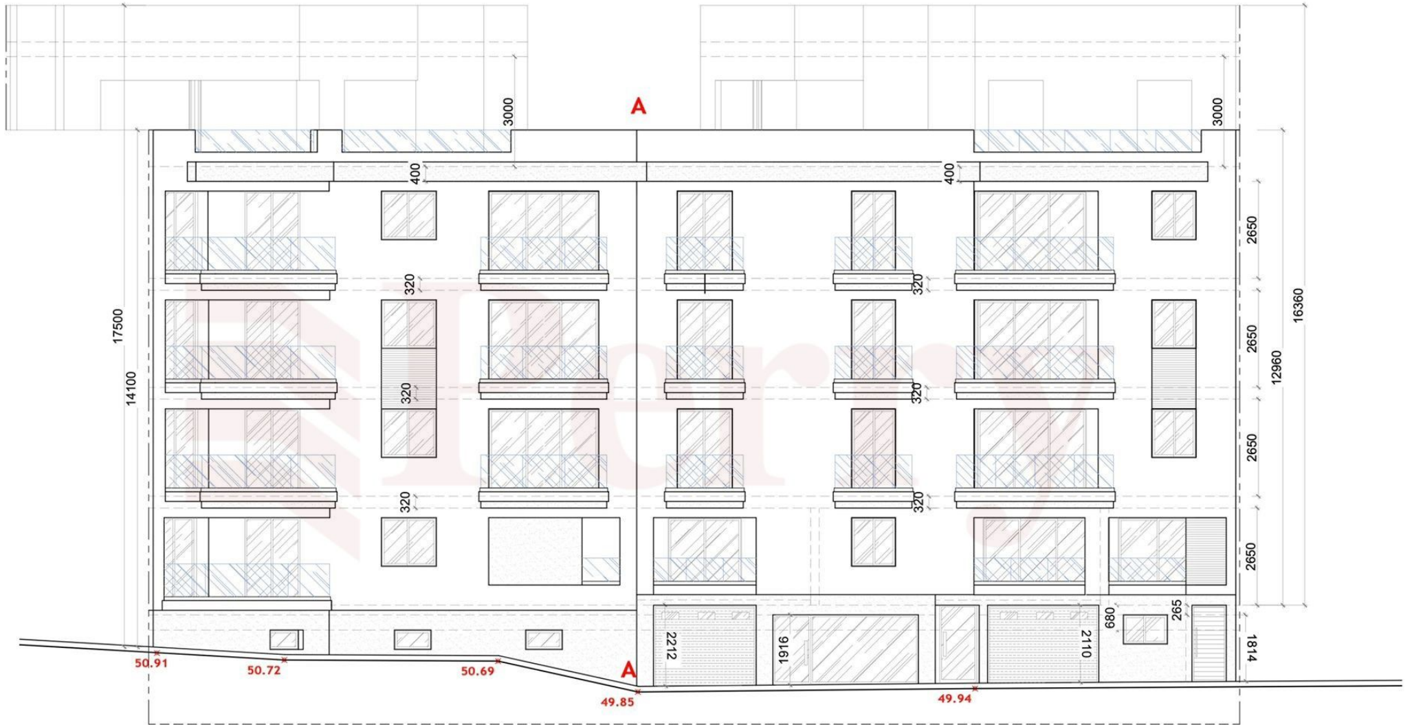
PROPOSED ELEVATION SCALE 1:100
