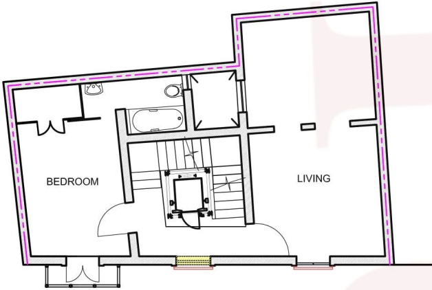
SECOND FLOOR PLAN SCALE 1/100
