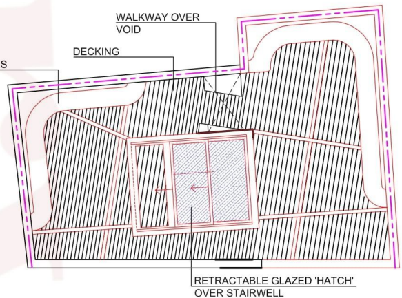
PROPOSED ROOF PLAN SCALE 1/100
