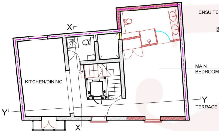
PROPOSED FOURTH FLOOR PLAN SCALE 1/100
