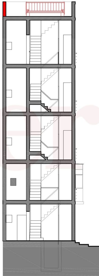
SECTION X-X SCALE 1/100
