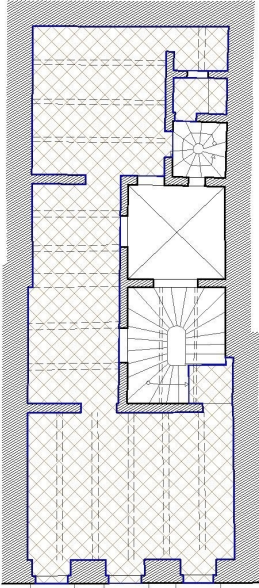
EXISTING 3RD FLOOR PLAN TOTAL INTERNAL FLOOR AREA (NET) - 67 SQM
