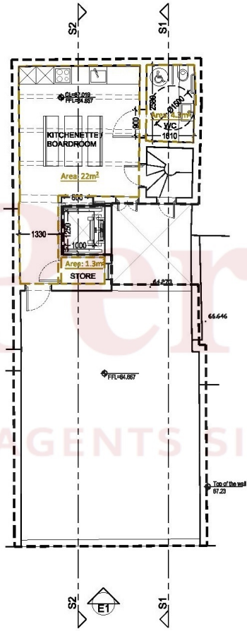
PROPOSED 4TH FLOOR LEVEL (EXTENSION) GROSS FLOOR AREA PER FLOOR: 95 sqm
