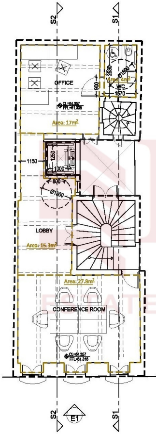
PROPOSED 3RD FLOOR GROSS FLOOR AREA PER FLOOR: 94 sqm
