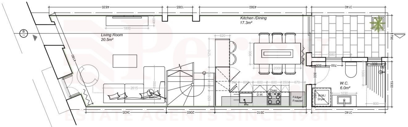
5 Proposed Plan Ground Floor SCALE 1:50
