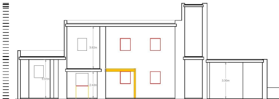
SECTION B-B as PROPOSED SCALE 1:100
