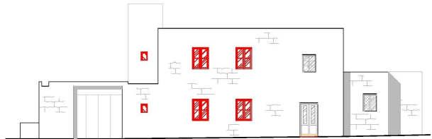
ELEVATION as PROPOSED SCALE 1:100
