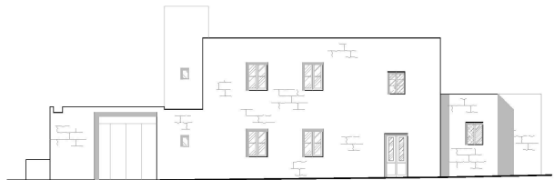
ELEVATION SCALE 1:100
