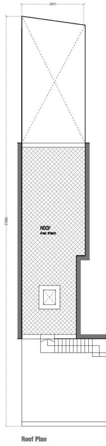
Roof Plan
