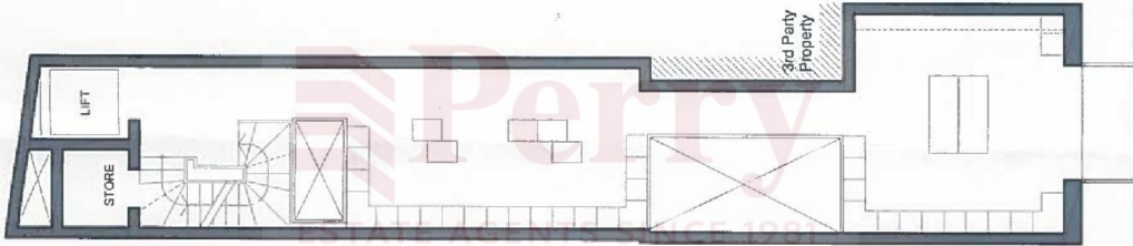
Proposed Second Floor Plan Scale 1:50 @ A1 Gross Floor Area: 75 sq. m.
