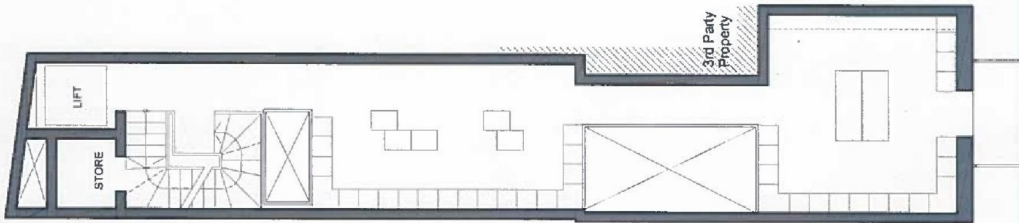
Proposed First Floor Plan Scale 1:50 @ A1 Gross Floor Area: 75 sq. m.
