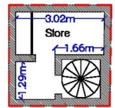
INTERMEDIATE FLOOR PLAN AREA: 12 SQ.M.
