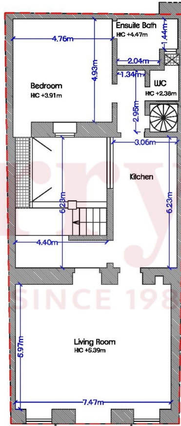
THIRD FLOOR PLAN AREA: 164 SQ.M.
