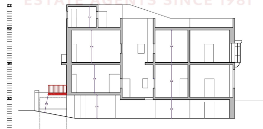
PROPOSED SECTION Y-Y Scale: 1/100
