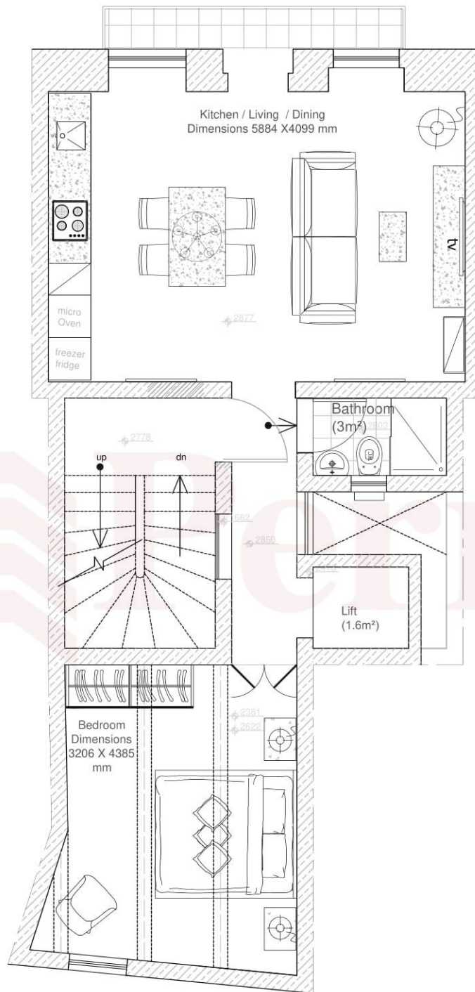
○ Third Floor
