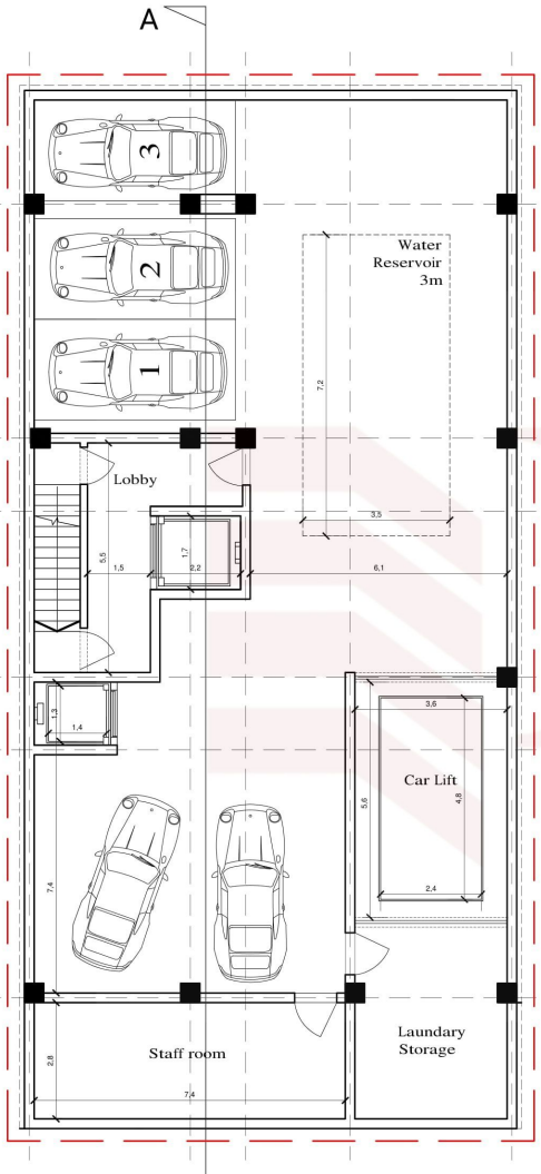
Proposed Basement Plan Level -3/ -4/ CLASS 3A
