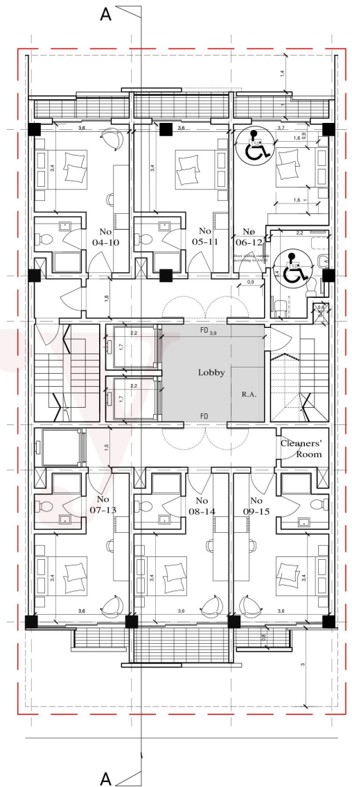
Proposed Floor Plan with 1 Accessible Room Level +2/ +3 CLASS 3A
