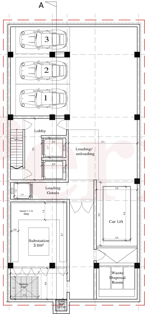
Proposed Basement Plan Level -2 CLASS 3A
