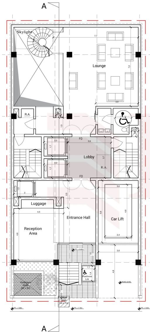
Proposed Ground Floor Plan Level 0 CLASS 3A
