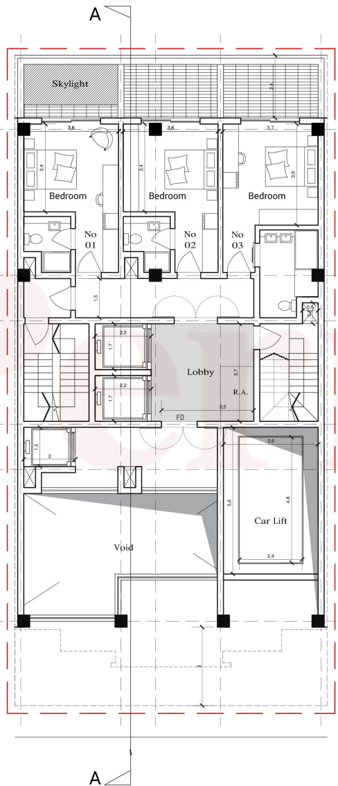
Proposed First Floor Plan Level 1 CLASS 3A
