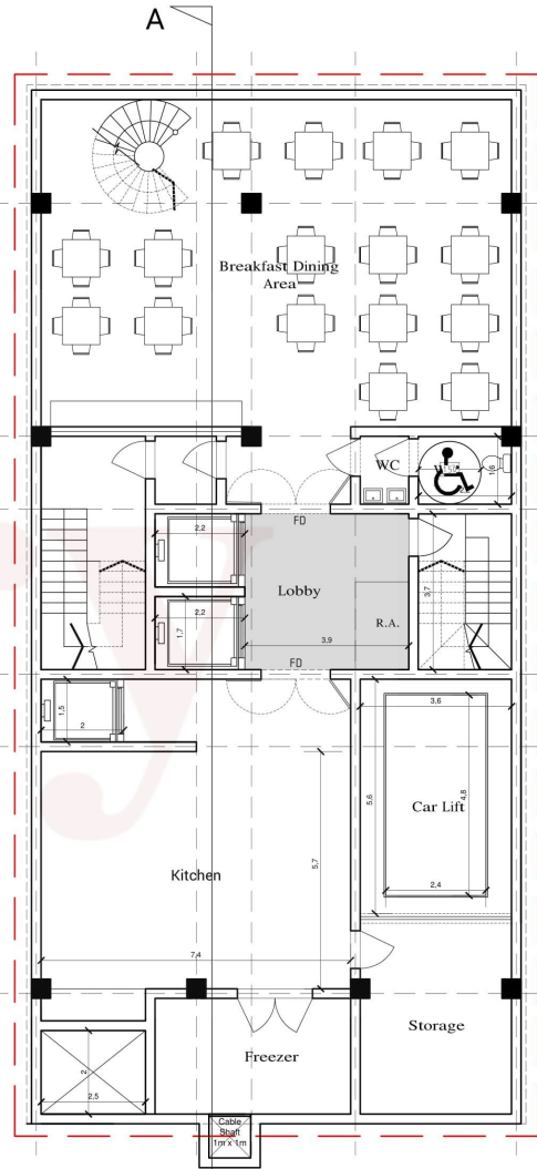
Proposed Basement Floor Plan Level -1 CLASS 3A
