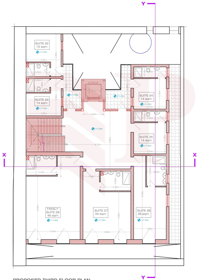
PROPOSED THIRD FLOOR PLAN Scale:- 1:100
