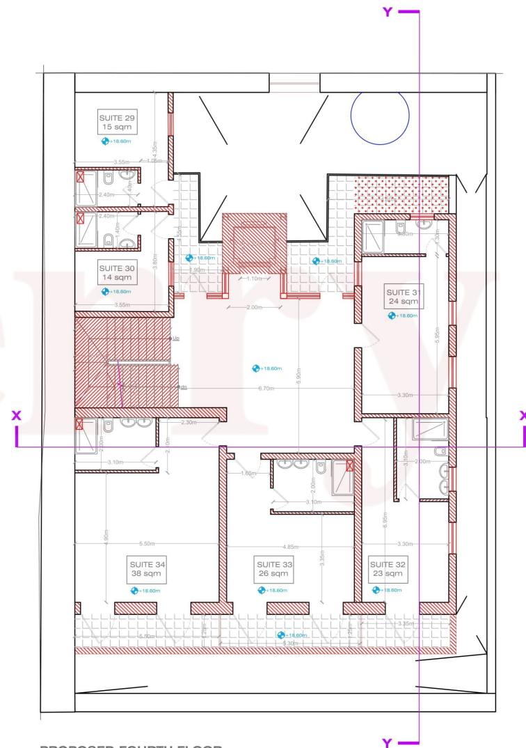
PROPOSED FOURTH FLOOR PLAN Scale:- 1:100
