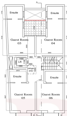
Proposed First Floor Plan Scale 1:100
