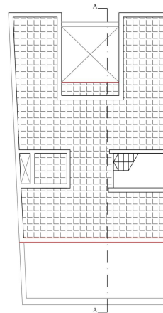
Proposed Roof Plan Scale 1:100
