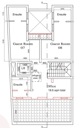
Proposed Second Floor Plan Scale 1:100
