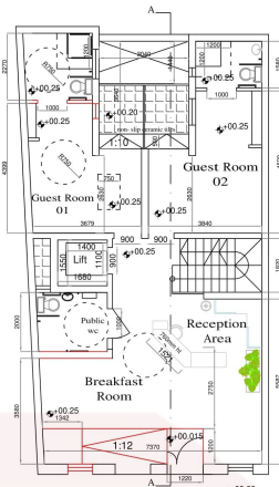
Proposed Ground Floor Plan Scale 1:100
