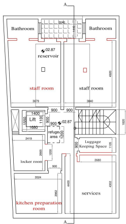
Proposed Basement Floor Plan Scale 1:100
