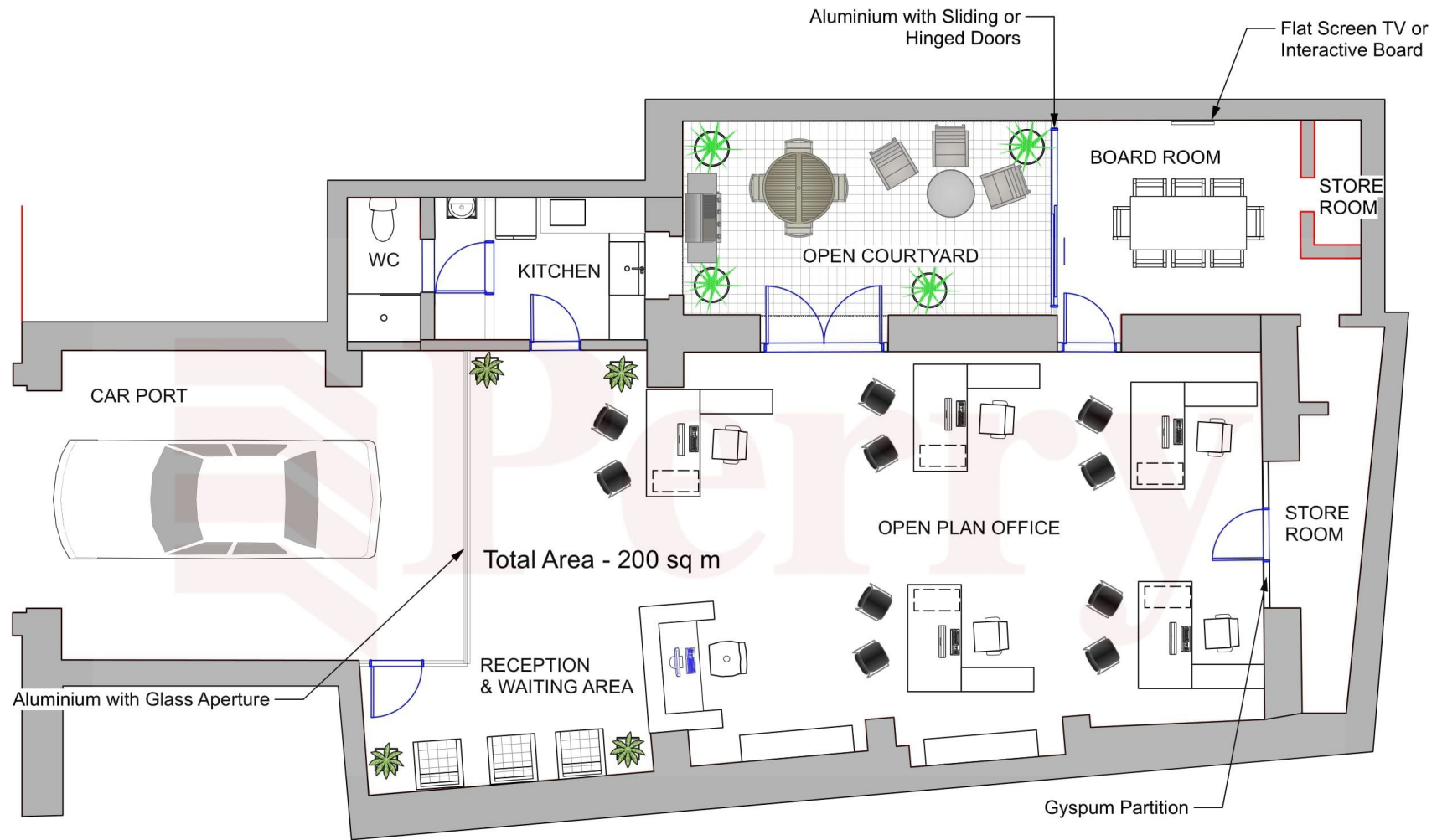
1 Proposed Ground Floor Office Floor Plan Scale: 1:75
