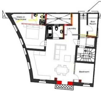
PROPOSED FOURTH FLOOR PLAN Scale: 1:100 SUPERIMPOSED
