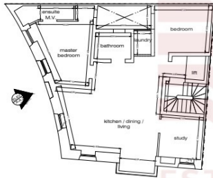
APPROVED FIRST FLOOR PLAN - (93m 2 ) Scale - 1:100
