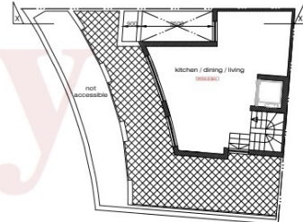
PROPOSED SIXTH FLOOR PLAN Scale: 1:100 CLEAN-COPY
