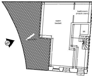
APPROVED GROUND FLOOR PLAN - (53m 2 ) Scale - 1:100
