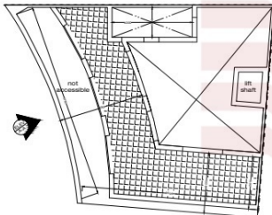
APPROVED upper 5th FLOOR PLAN - (67m 2 ) (double volume) Scale: 1:100
