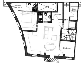
PROPOSED FOURTH FLOOR PLAN Scale: 1:100 CLEAN-COPY
