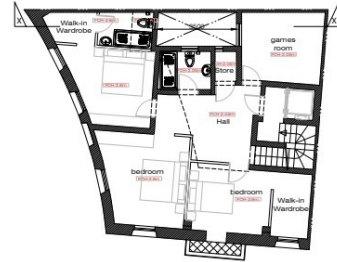
PROPOSED FIFTH FLOOR PLAN Scale: 1:100 CLEAN-COPY
