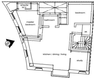
APPROVED 2nd, 3rd & 4th FLOOR PLAN - (93m 2 ) Scale - 1:100
