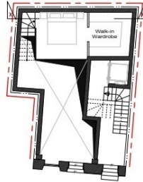
PROPOSED INTERMEDIATE GROUND FLOOR PLAN Scale - 1:100 SUPERIMPOSED
