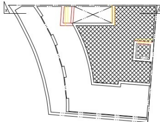
PROPOSED ROOF PLAN Scale: 1:100 SUPERIMPOSED
