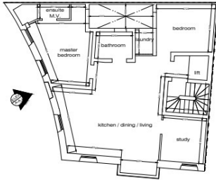
APPROVED 5th FLOOR PLAN - (93m 2 ) Scale: 1:100
