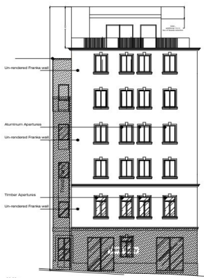
APPROVED ELEVATION A-A Scale: 1/100
