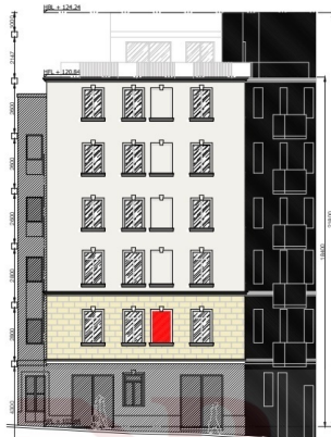
PROPOSED ELEVATION A-A Scale: 1/100 SUPERIMPOSED
