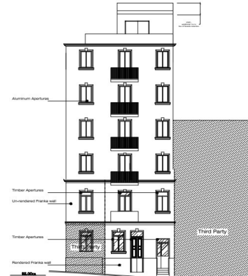
APPROVED ELEVATION B-B Scale: 1/100
