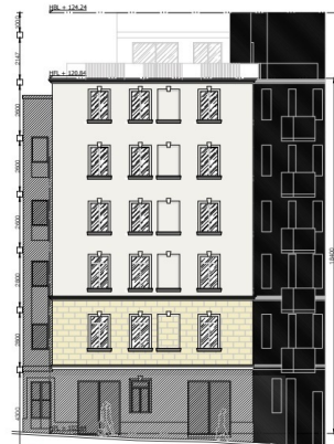
PROPOSED ELEVATION A-A Scale: 1/100 CLEAN COPY
