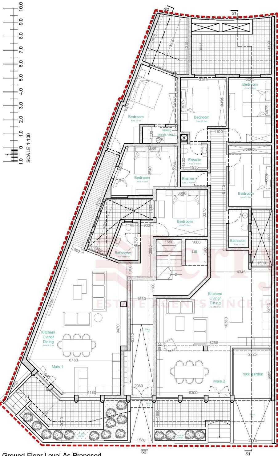
Ground Floor Level As Proposed
