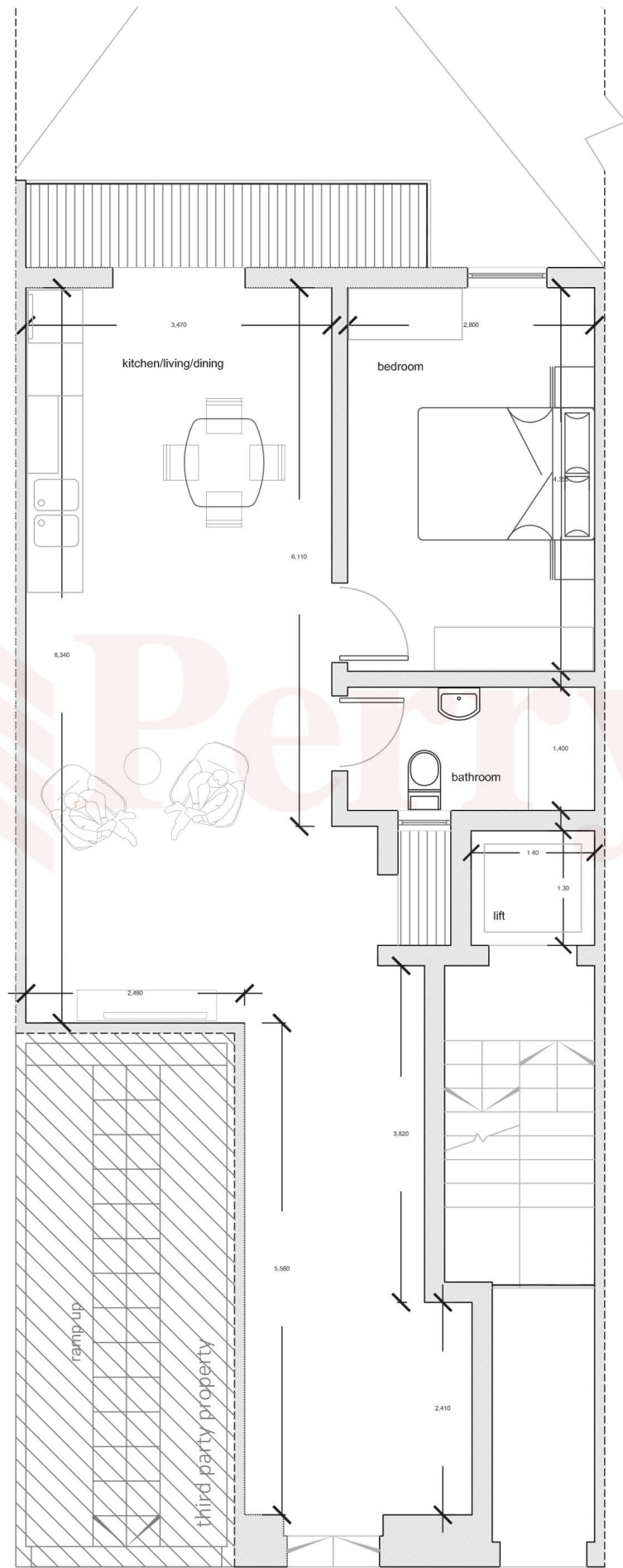
proposed ground floor - scale 1:50
