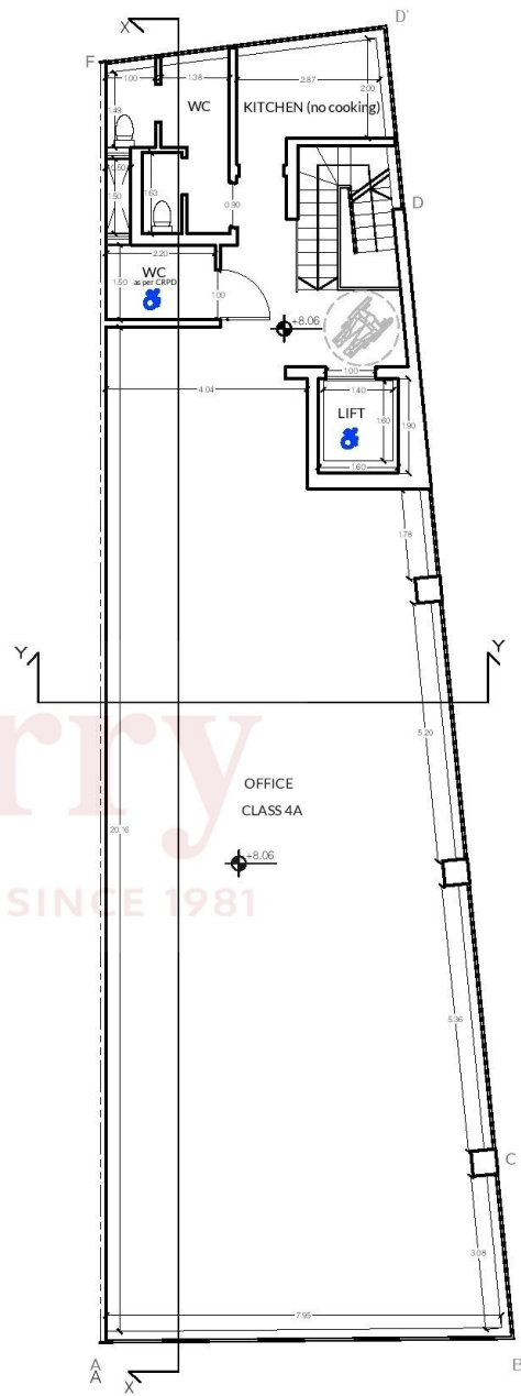
PROPOSED LEVEL 2 PLAN SCALE 1:100
