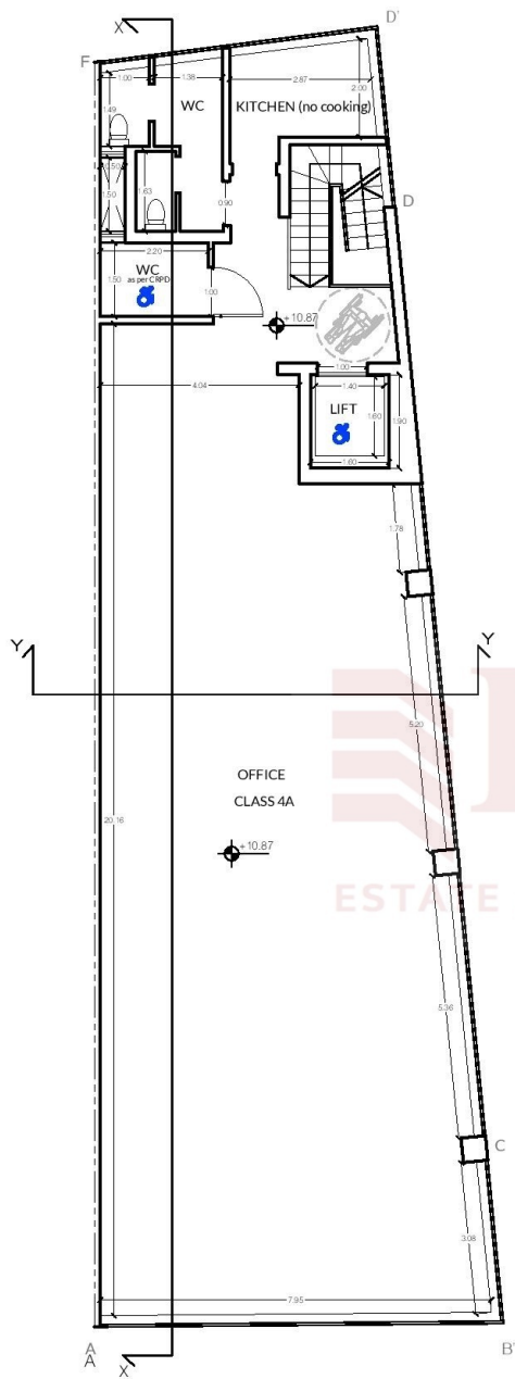
PROPOSED LEVEL 3 PLAN SCALE 1:100
