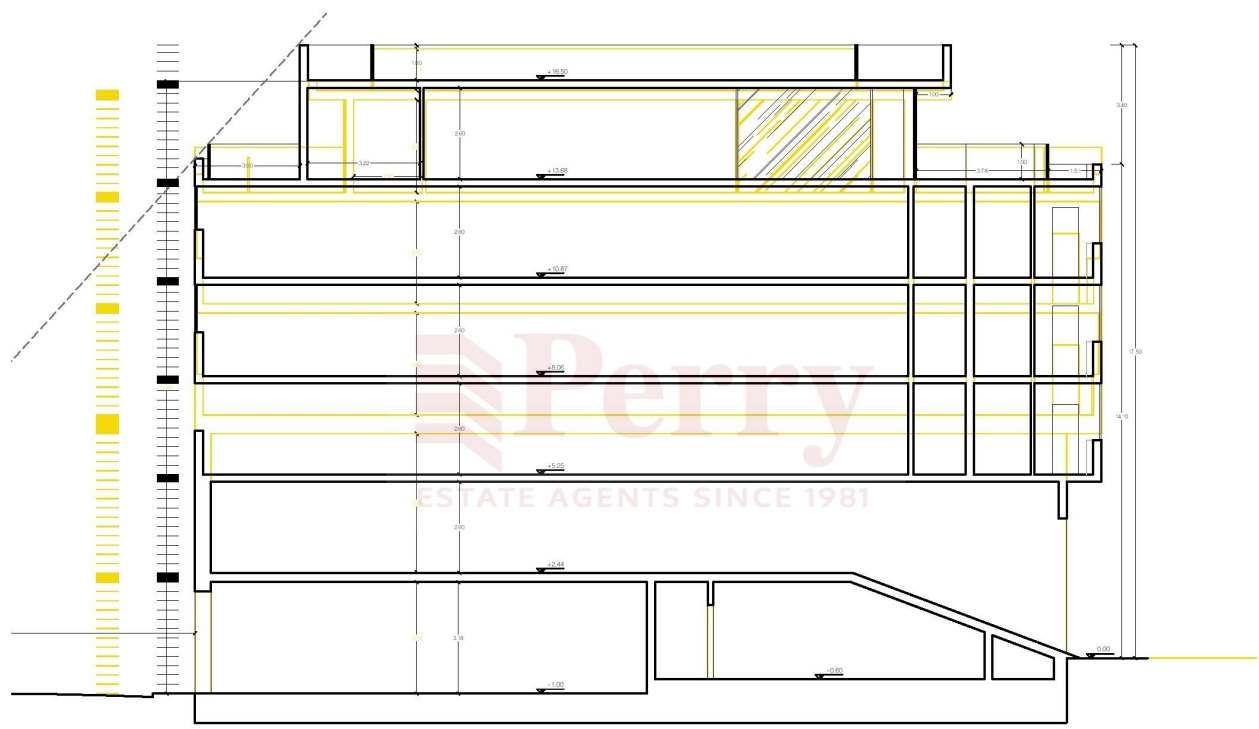
PROPOSED SECTION X-X SUPERIMPOSED PROPOSED SECTION WITH APPROVED ONE AS THE REASON/EXPLANATION OF DEMOLISHING SCALE 1:100
