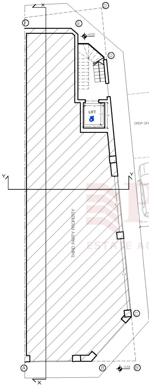
EXISTING SEMI-BASEMENT LEVEL PLAN SCALE 1:100
