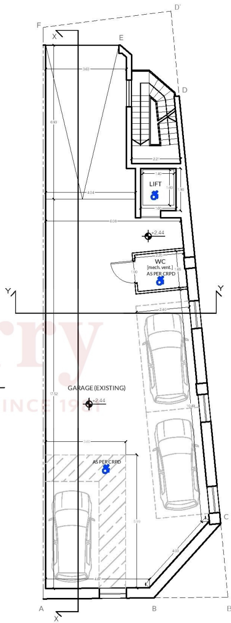
PROPOSED ELEVATED LEVEL 0 PLAN SCALE 1:100
