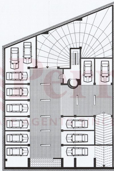
Plan Basement Level -1
