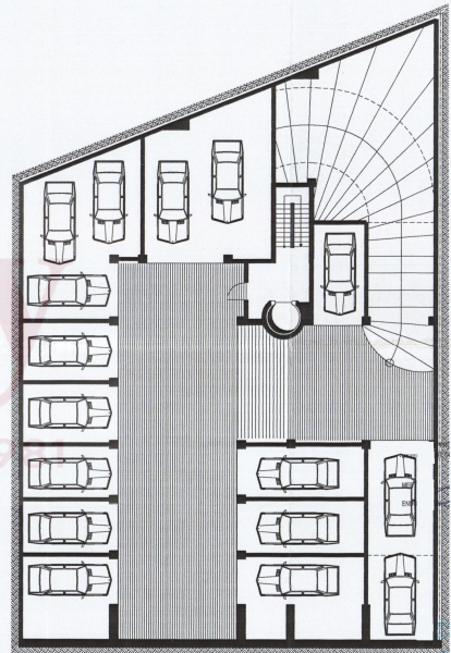
Plan Basement Level -2
