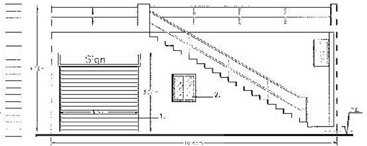
Front Elevation Proposed Scale 1:50
