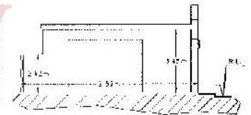
Section A - A Proposed Scale 1:25
