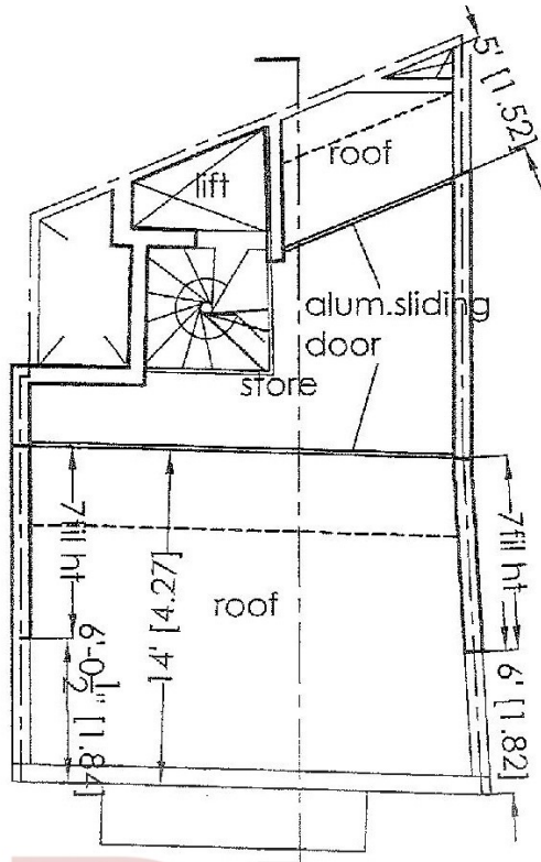
4th. Fl. Plan as amended
